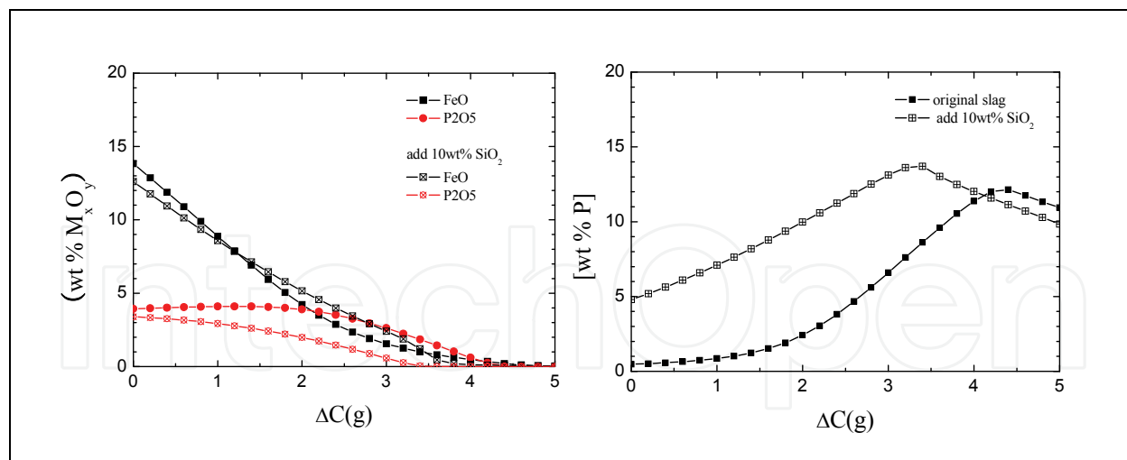
Fig. 4. Effect of \text{SiO}_2 addition on the change in the composition of (a) \text{FeO} and \text{P}_2\text{O}_5 in slag and (b) P in metal at 2073K by the carbothermic reduction. Initial slag weight is assumed to be 100g, and \Delta C is the amount of carbon consumption. (Lee et al. , 2010)
