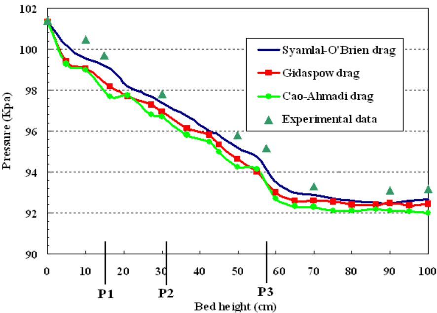
Fig. 7. Comparison of simulated pressure variation versus bed height using Cao-Ahmadi, Syamlal-O'Brien and Gidaspow drag models with the experimental data for a superficial velocity of V_g = 50 \text{ cm/s} and position of pressure transducers (P1, P2 and P3).
