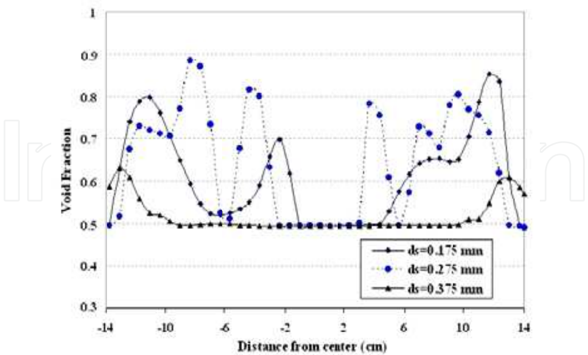
Fig. 17. Simulated void fraction at different solid particles diameter (at z=20 cm, U_g=38 cm/s, t=5.0 s)
