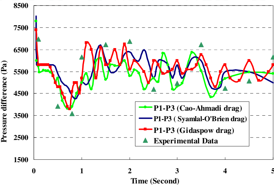
Fig. 6. Comparison of simulated bed pressure drop using different drag models with the experimental data for a superficial velocity of V_g = 50 \text{ cm/s} .
