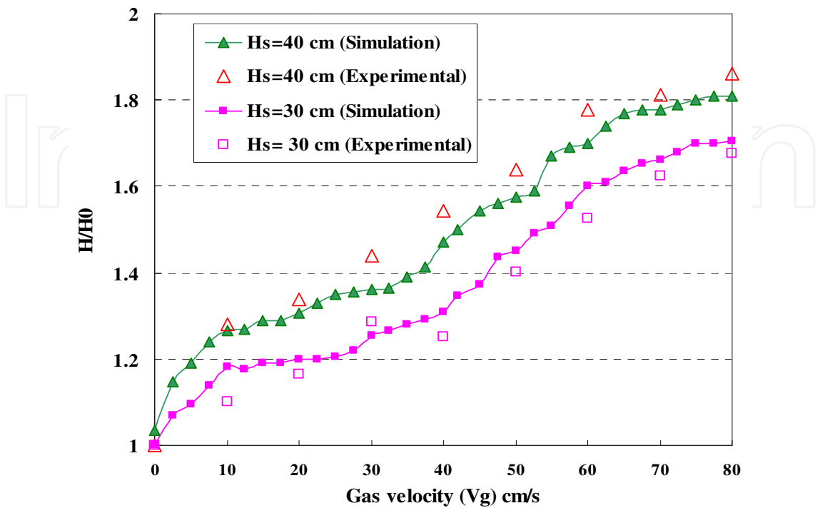
Fig. 16. Comparison of experimental and simulated bed expansion ratio for different initial static bed height.
