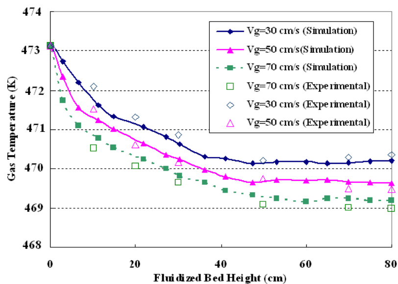
Fig. 34. Comparison of experimental and computational results of gas temperature at different gas velocity ( H_s=40 cm, t=5 s)
