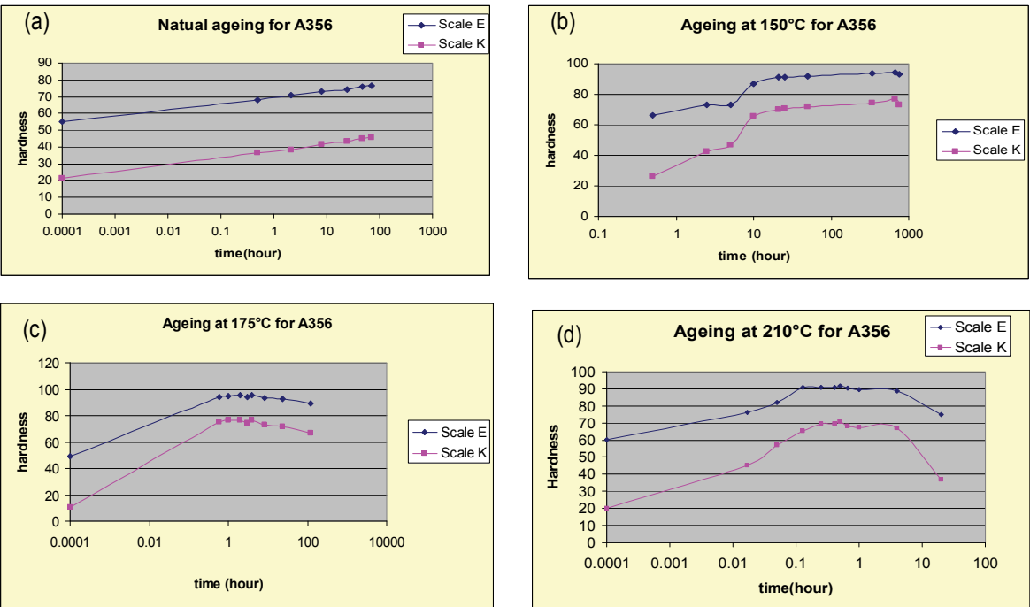
Fig. 4. Hardness changes with time for A356 at (a) Natural ageing; (b) 150^\circ\text{C} ; (c) 175^\circ\text{C} ; (d) 210^\circ\text{C}
