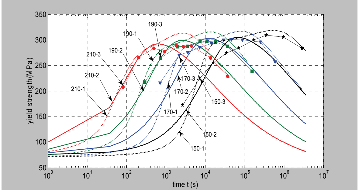
Fig. 11. Modelling of age hardening for A357 at ageing temperatures of 150°C, 170°C, 190°C and 210°C by Schercliff-Ashby method and KWN model, and comparasion with experimental data.
