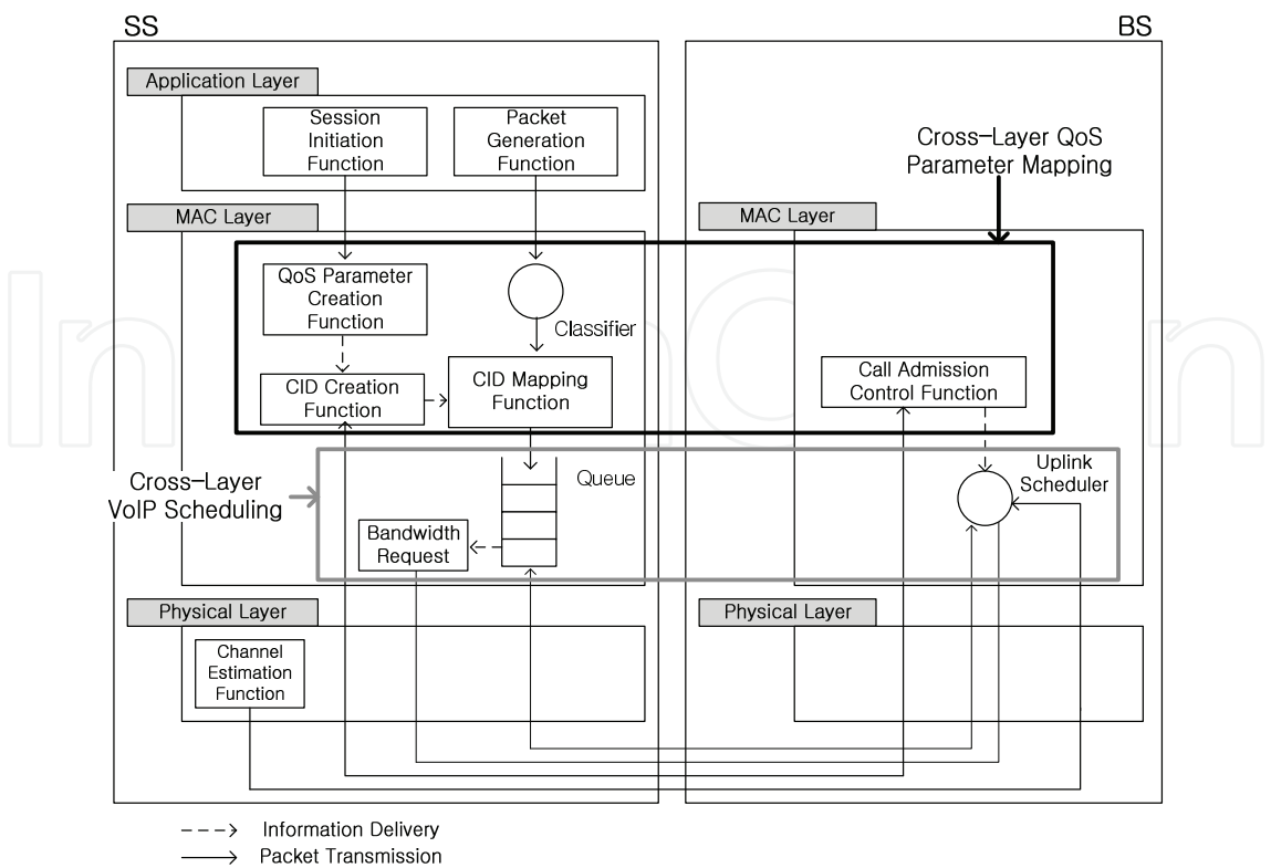
Fig. 4. Cross-layer framework for VoIP services
