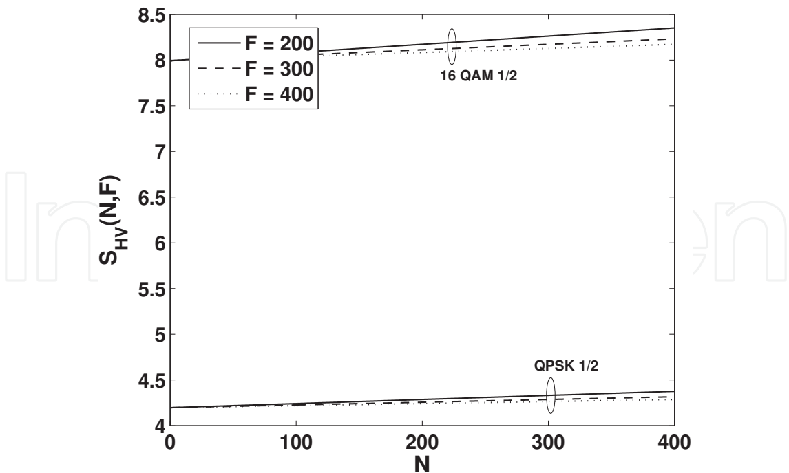
Fig. 8. S_{HV}(N,F) vs. N and F (MCS level = QPSK 1/2 and 16 QAM 1/2, VoIP speech codec = EVRC, S_{TOT} = 144 slots, T_{MF} = 5 msec, FFT size = 1024, \lambda = 2.5 , \mu = 1.67 , and bandwidth = 10 MHz)
