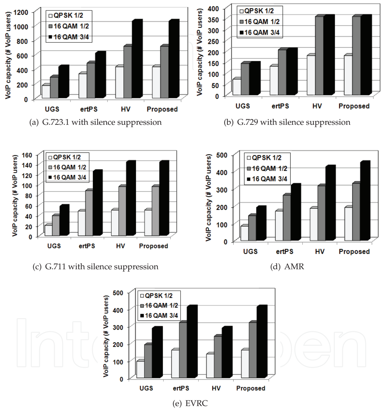
Fig. 9. VoIP capacity vs. VoIP scheduling algorithms and MCS levels ( S_{TOT} = 144 slots, T_{MF} = 5 msec, FFT size = 1024, \lambda = 2.5 , \mu = 1.67 , compressed RTP/UDP/IP header size = 3 bytes and bandwidth = 10 MHz)
