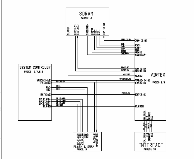
Fig. 33. PCB Bloc diagram of the VOIP Gateway
