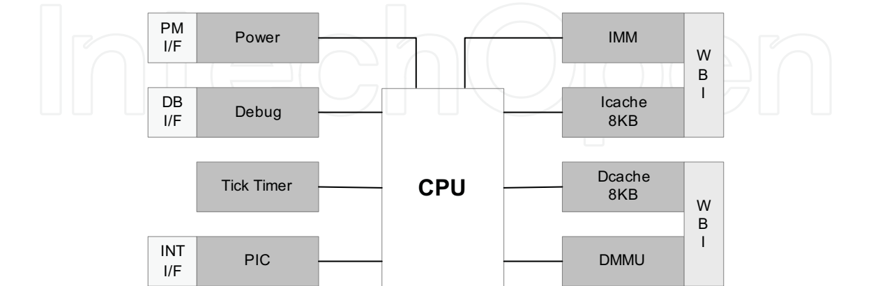
Fig. 13. The OpenRISC 1200 architecture
