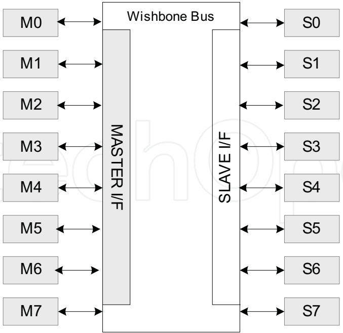
Fig. 12. Wishbone configuration
