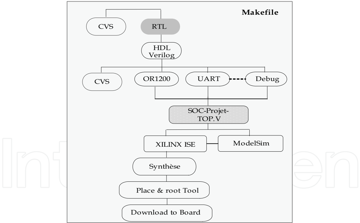
Fig. 7. Structured Makefile
