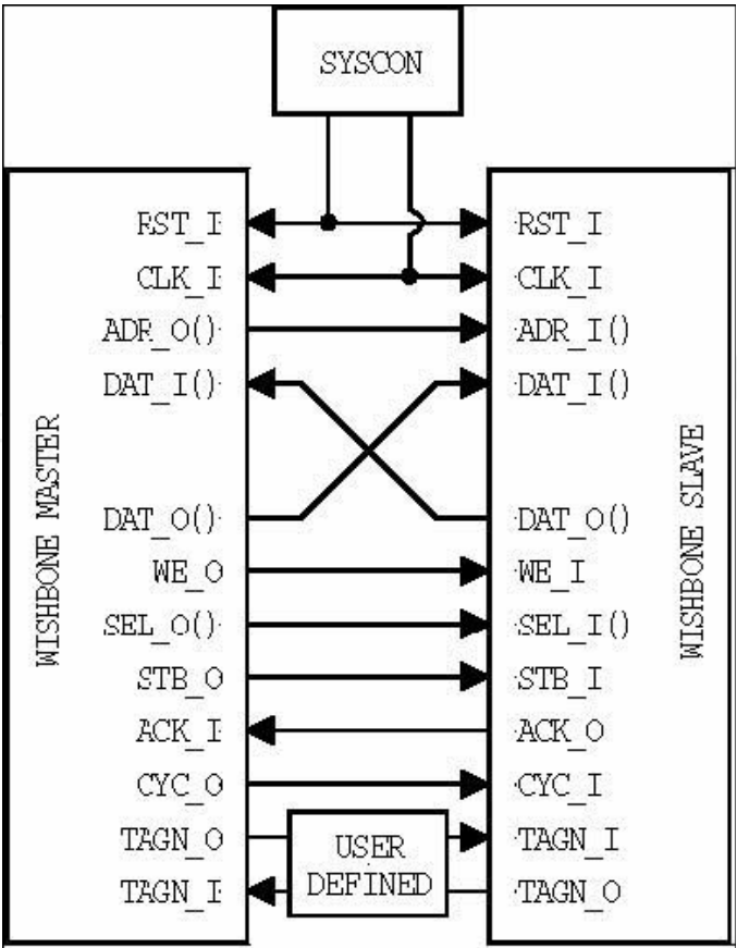
Fig. 11. Wishbone interconnection
