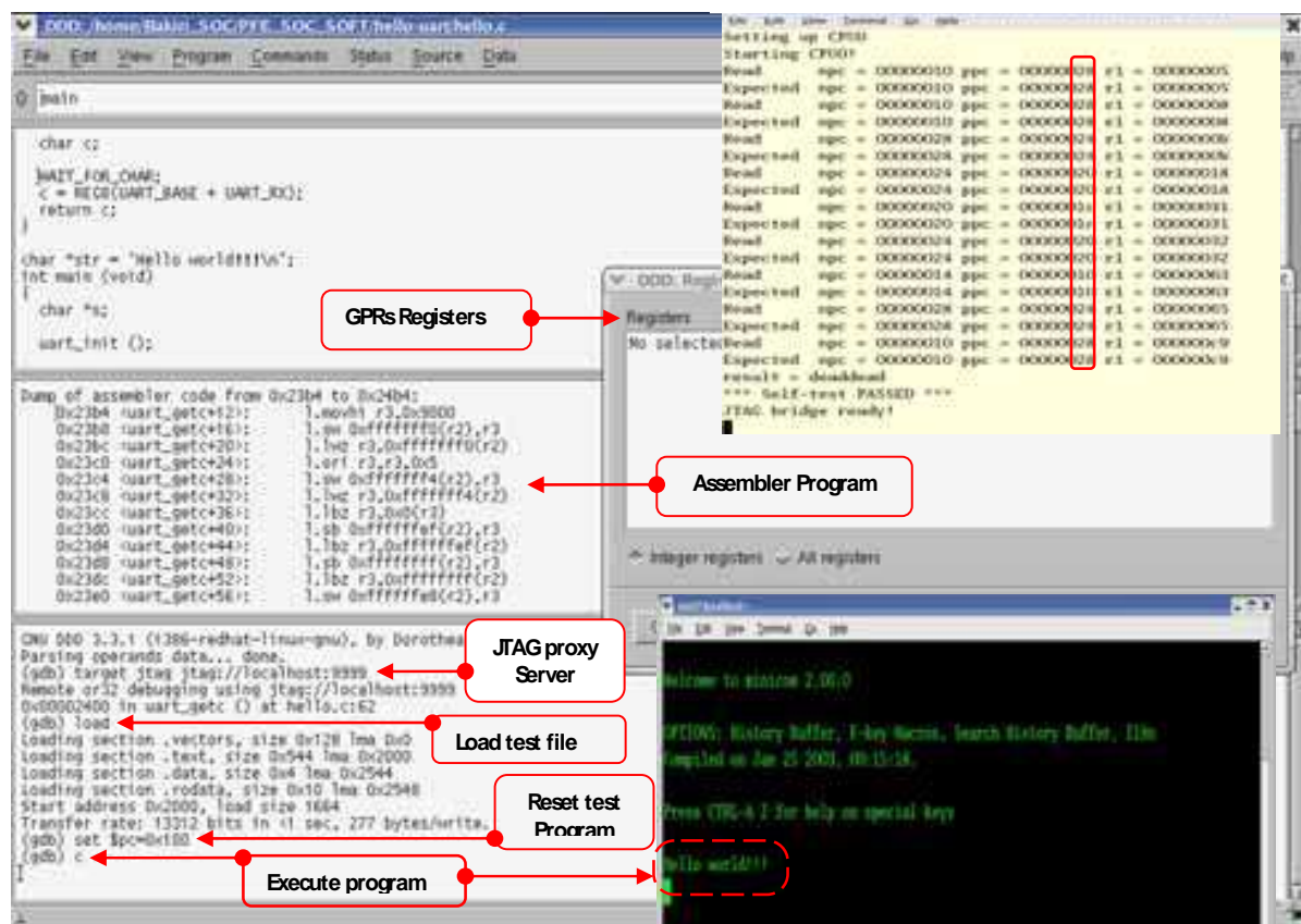
Fig. 28. Results of the serial transfer test
