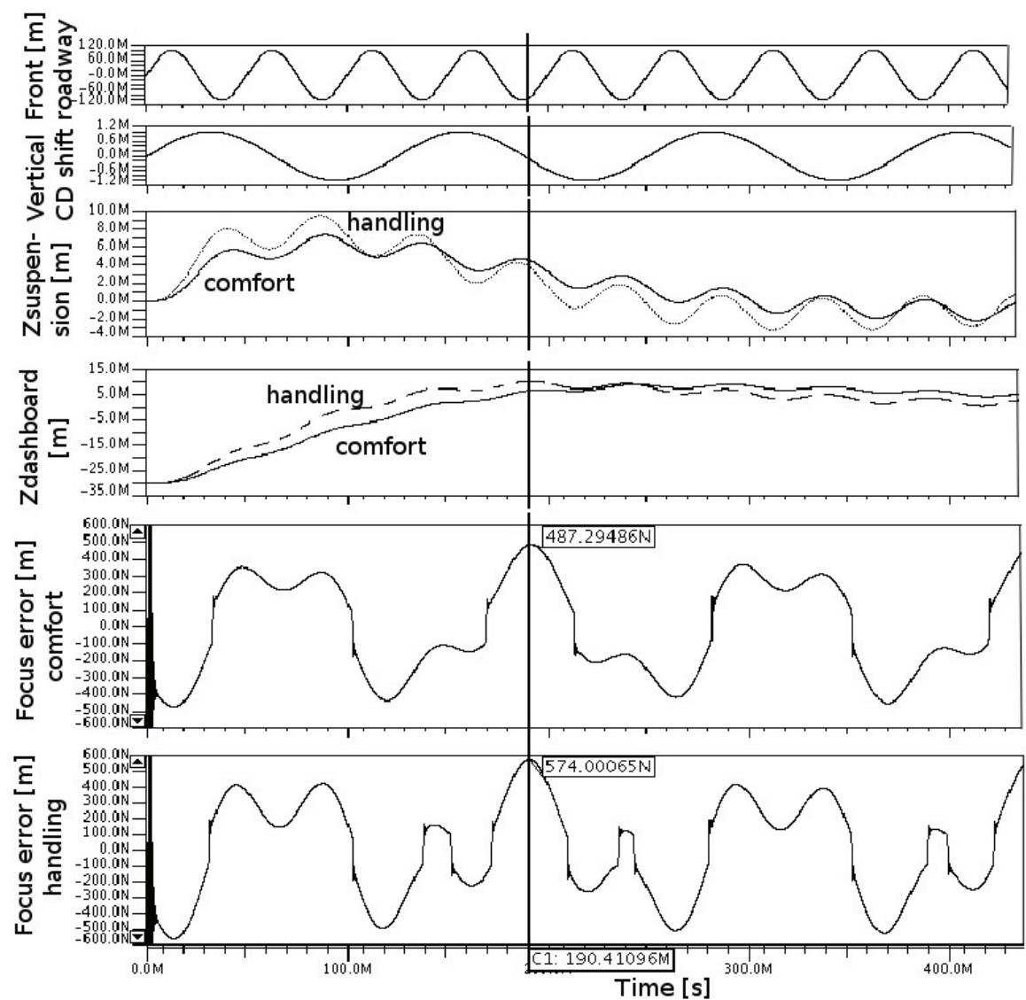
Fig. 17. CD player focus error for suspension parameters in the case of a comfort and a handling vehicle. The roadway profile is changing in a sinusoidal way in both the front and the back of the vehicle. Sine roadway profile (front an back): 0.1m peak, 25Hz. CD vertical shift max 1mm.
