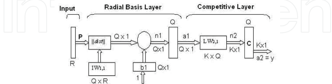
Fig. 3. The architecture of probabilistic network
