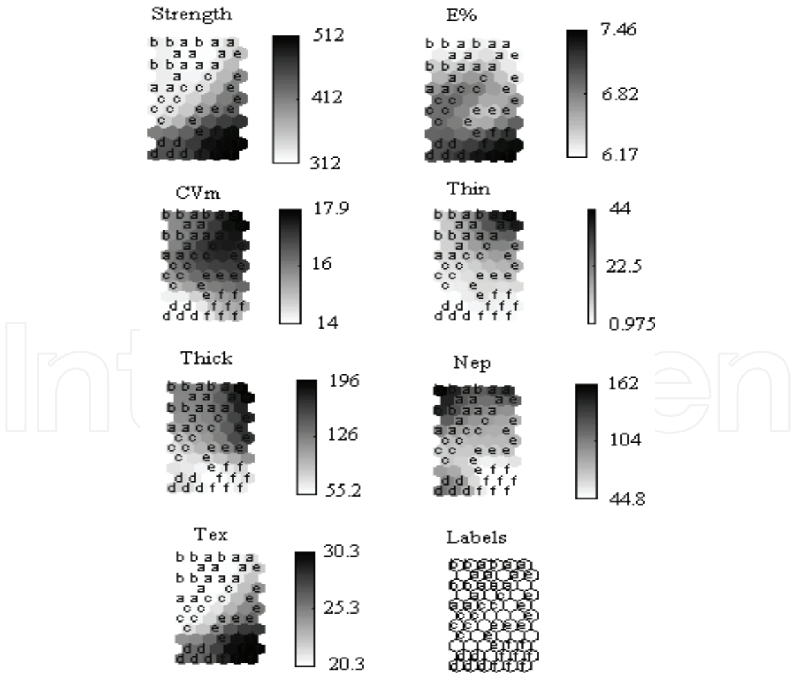
Fig. 15. The Quality Characteristics of Kenyan Cotton
