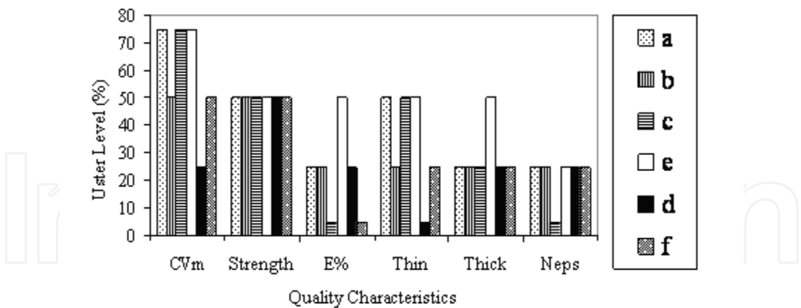
Fig. 11. Uster Standards for Kenya Cotton Yarn
