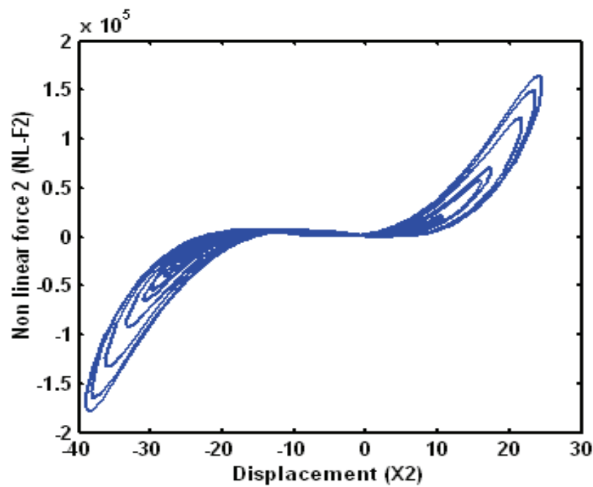
Fig. 14b. Nonlinear forces (X2, NL-F2) "Generalized case: quadratic and cubic for week damping"
