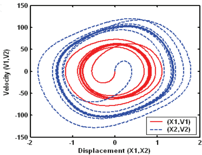
Fig. 5b. Phase diagrams "Van Der Pol case" Consequently, the phase diagram for each dof (figure 5b) indicates a cycle limit meaning stability, these two cycles are complementary.
