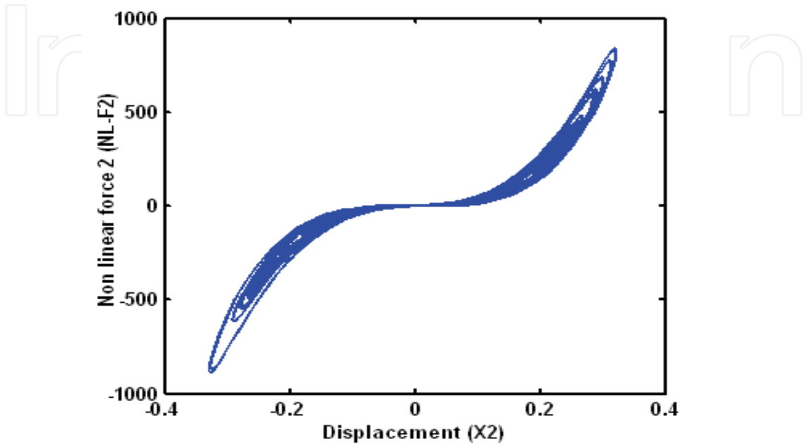
Fig. 3b. Nonlinear forces: (X2, NL-F2) "Duffing case"
