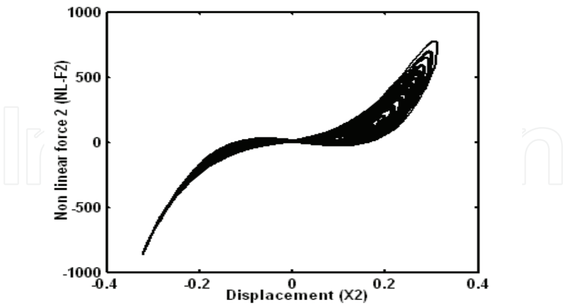
Fig. 9b. Nonlinear forces (X2, NL-F2) "Cubic damping and stiffness case"
