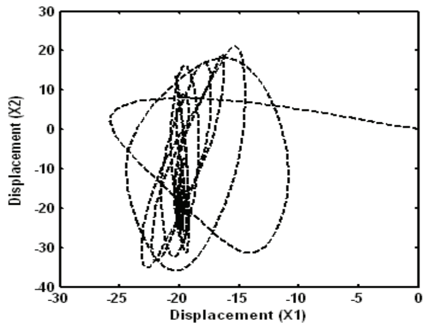
Fig. 15a. System trajectory in the plan (X1, X2) "Generalized case: quadratic and cubic for week damping"
