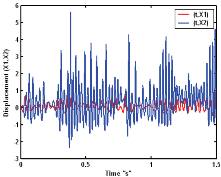
Fig. 19. Temporal nonlinear responses: (X_1(t)) and X(t) "Generalized case: power 1.5 and cubic for weak damping" Figure 19 shows the displacements evolution for the two dof according to time. It is noted that the auxiliary system completely absorbs the vibration in this proportioning configuration. It is as to note as the movement is relatively irregular similar of specified non linearity. That may be one of the effects of the generalized non linearity for the non integer power less then 2.
