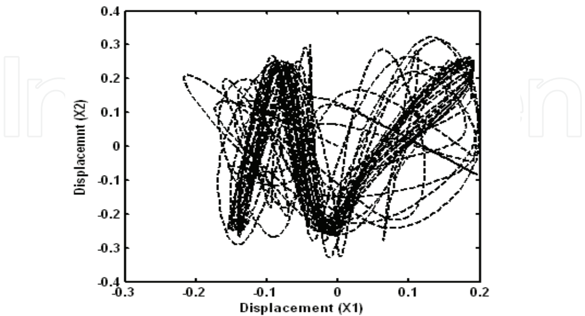
Fig. 4a. System trajectory in the plan (X1, X2) "Duffing case"
