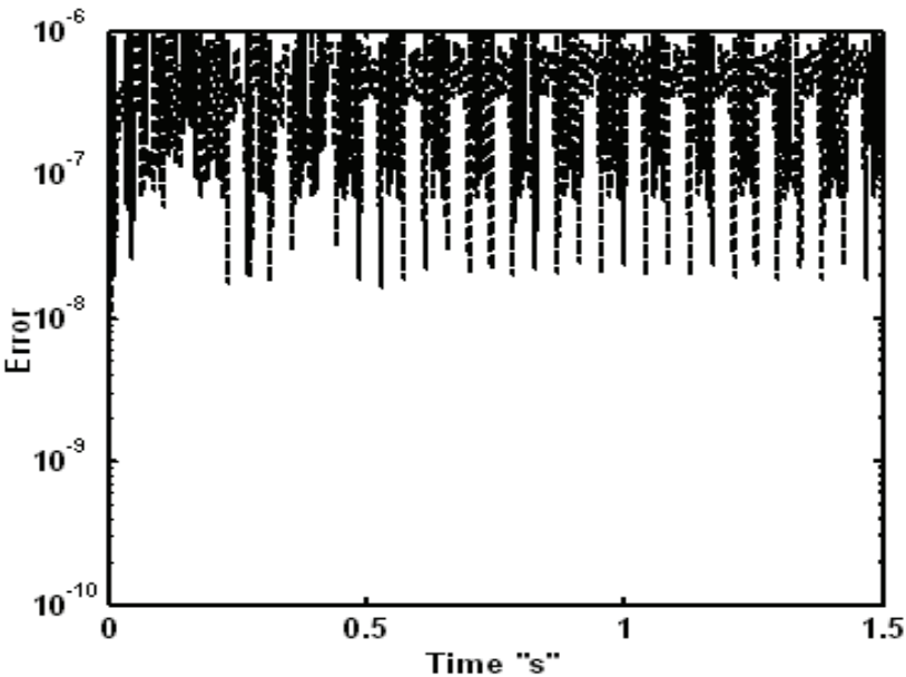
Fig. 7b. Error curve "Van Der Pol case"
