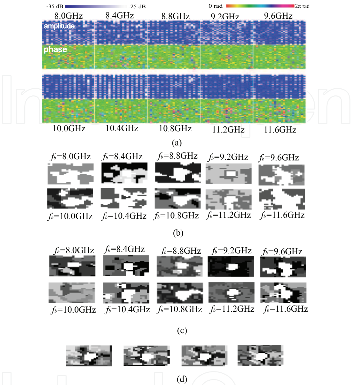
Fig. 8. Experimental results 2 for heavily wet laterite soil. (a)Amplitude and phase images at 10 frequency points, (b)classification results with the previous method. Numbers denote base frequency f_b , (c)classification results with utilization of SOM-space topology in the CSOM. Numbers denote base frequency. (d)Classification results with utilization of SOM-space topology in the CSOM and frequency-domain local correlation method. The four images show the results with various initial reference vectors in the CSOM (Nakano & Hirose, 2009b).
