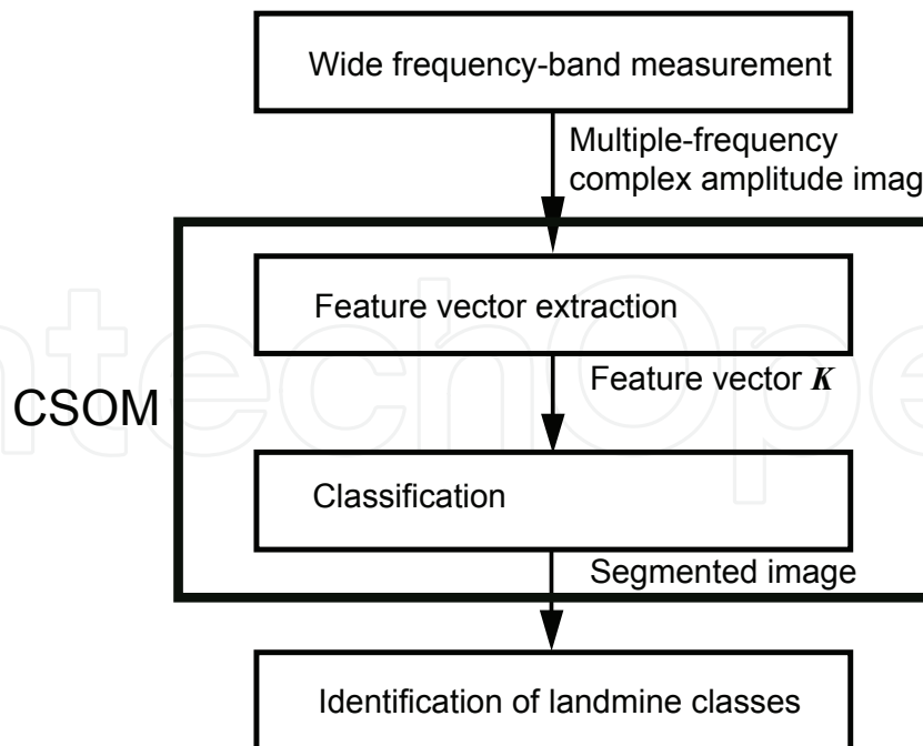
Fig. 2. The overall processing flow (Nakano & Hirose, 2009b).
