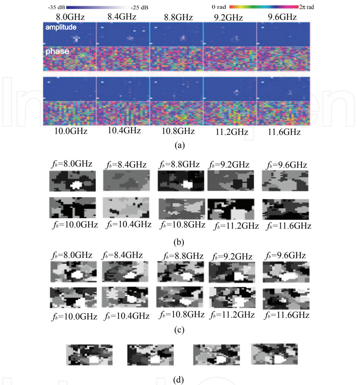
Fig. 7. Experimental results 1 for lightly wet laterite soil. (a)Amplitude and phase images at 10 frequency points, (b)classification results with the previous method. Numbers denote base frequency f_b , (c)classification results with utilization of SOM-space topology in the CSOM. Numbers denote base frequency. (d)Classification results with utilization of SOM-space topology in the CSOM and frequency-domain local correlation method. The four images show the results with various initial reference vectors in the CSOM (Nakano & Hirose, 2009b).
