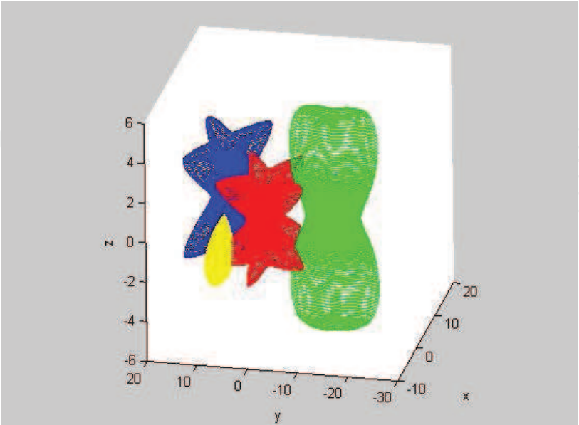
(b) NDOs represented in (x,y,z)
