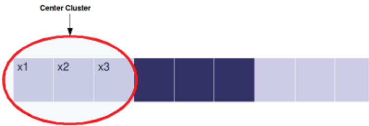
Fig. 11. Genome of the individual ( nc = 3 and N = 3 )
