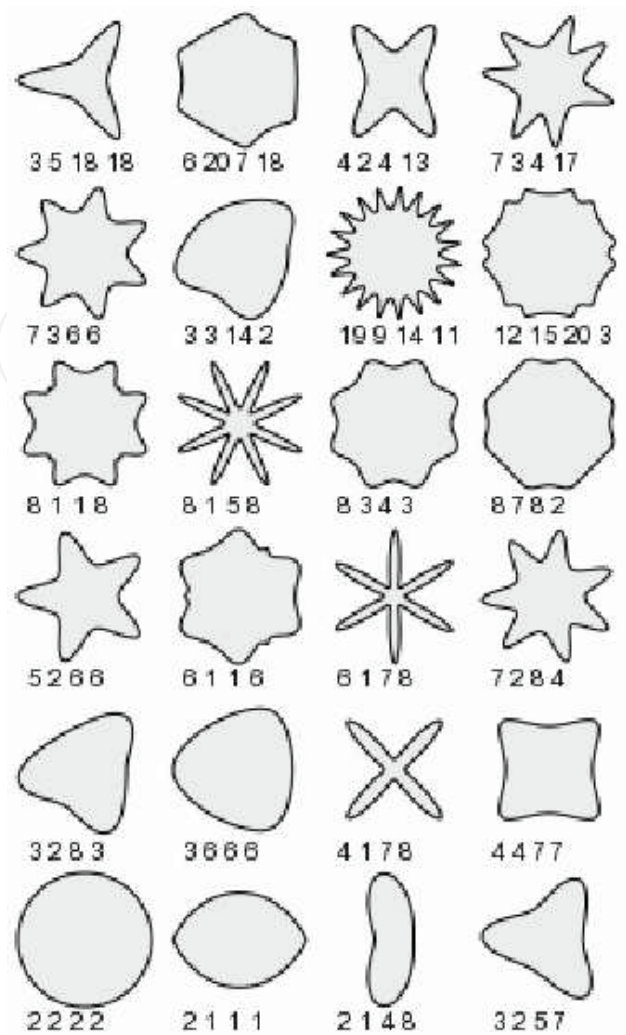
Fig. 6. Shapes in 2D generated by the Giellis equation
