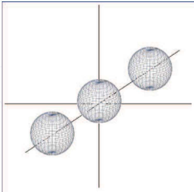
Fig. 3. Disjoint spherical clusters
