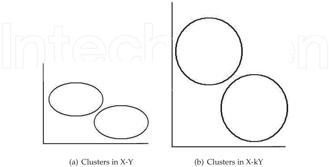
Fig. 2. Hypothetical clustering
