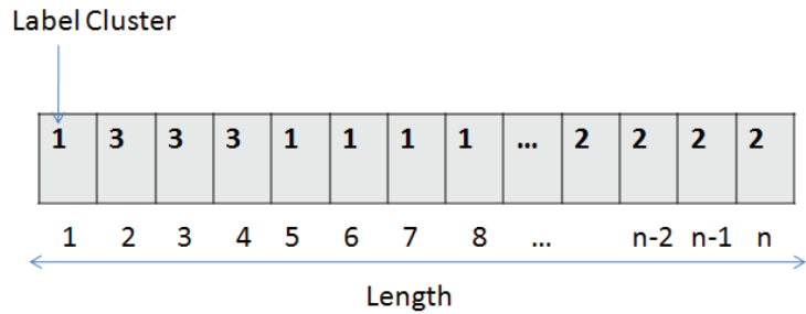
Fig. 15. Genome of the individual (k=3)
