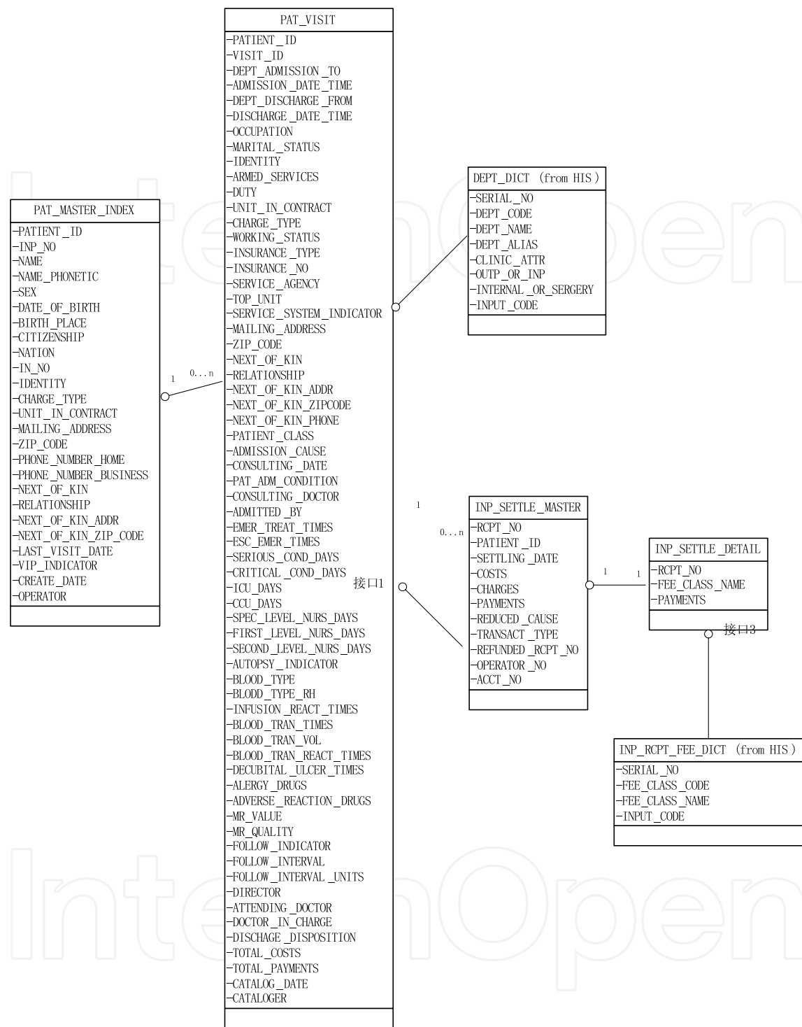
Fig. 6.5 Object model of inpatient fees This model will be analyzed in three aspects: medical insurance fee, department annual fee and fee compositions.
