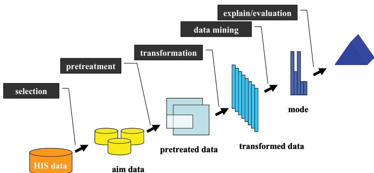
Fig. 3.1 KDD process
