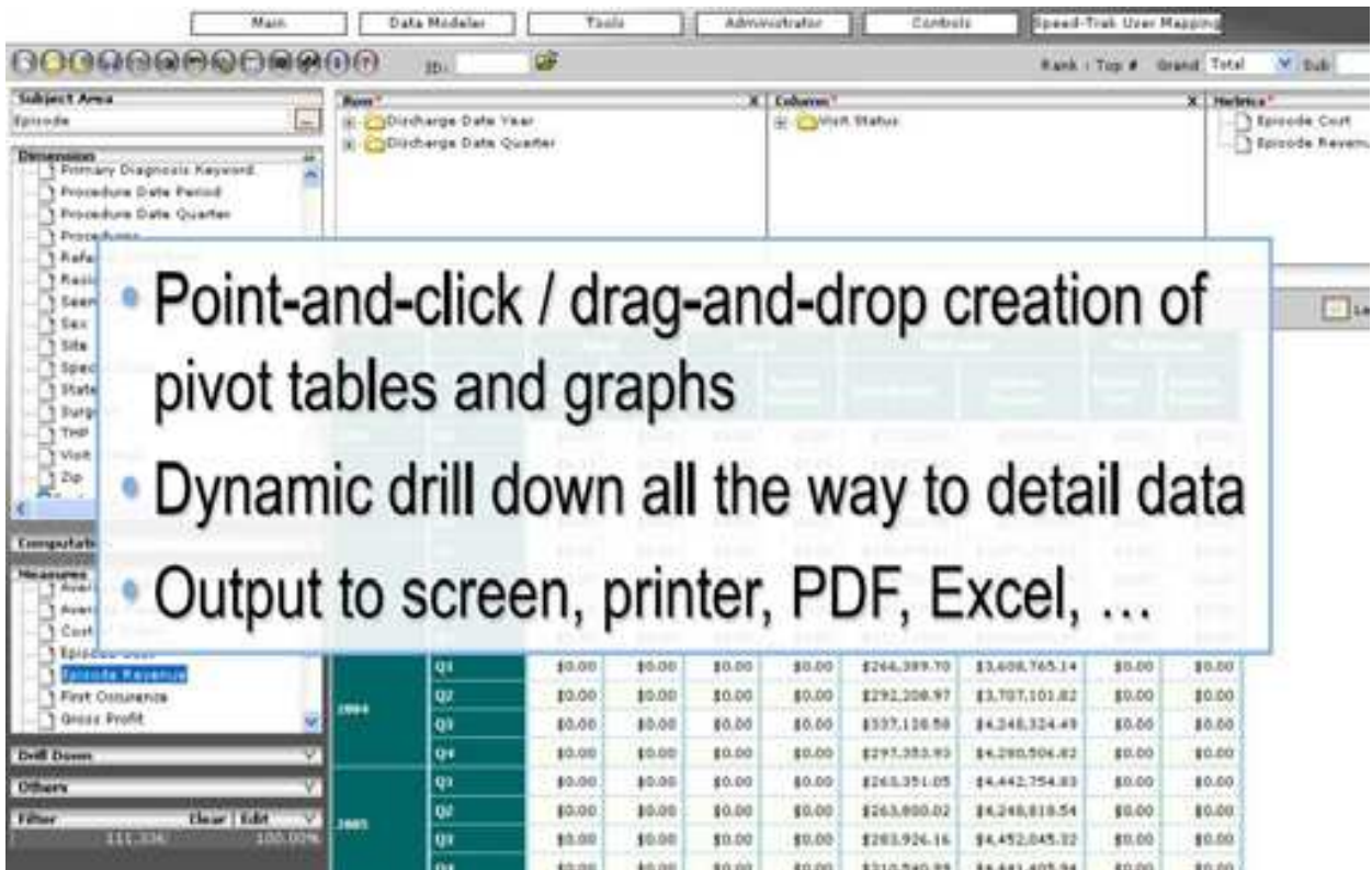
Fig. 6.3 DeepSee Analyzer
