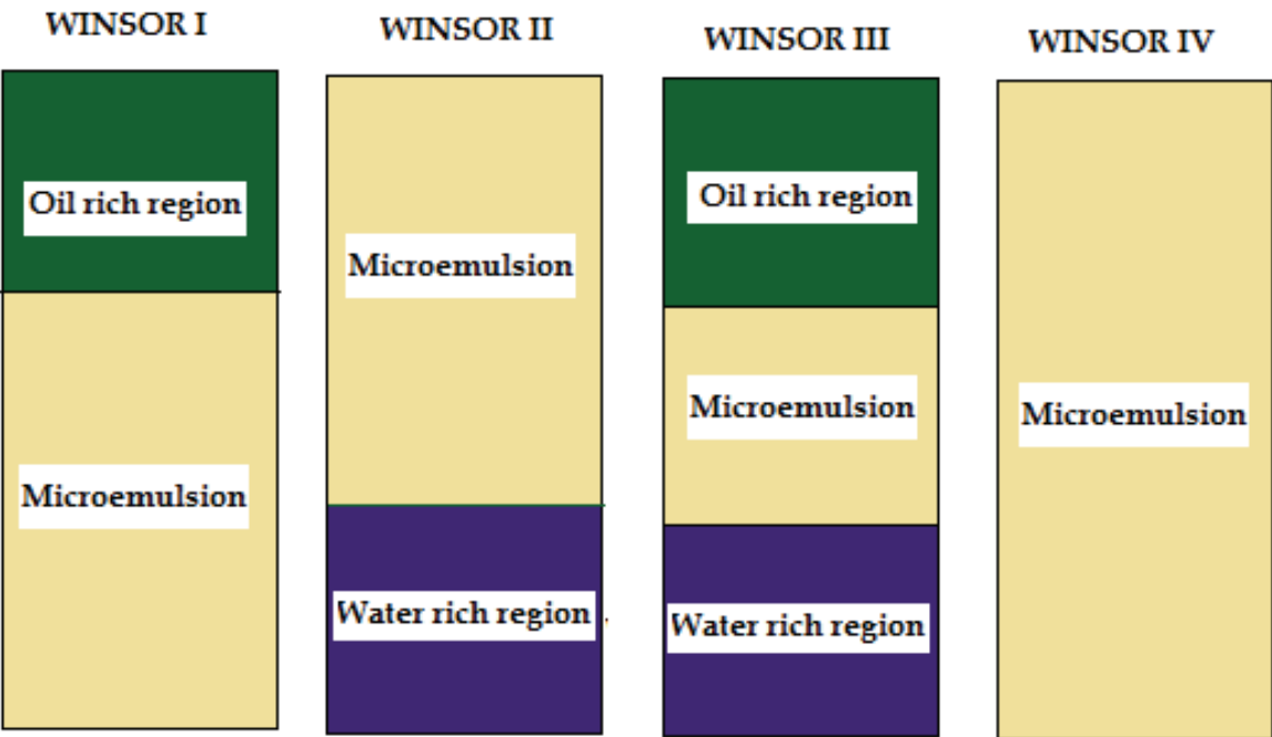
Fig. 2. Schematic presentation of most occurred surfactant associates
