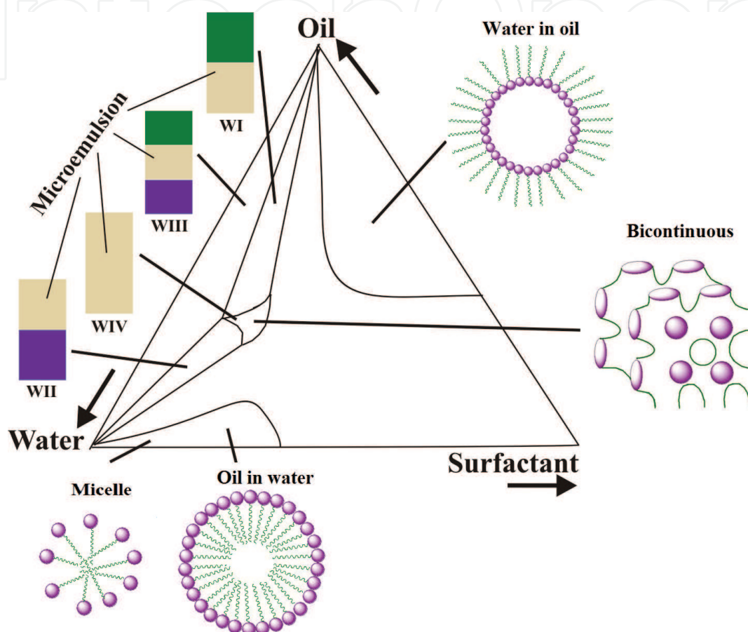
Fig. 1. A hypothetical ternary phase diagram representing three components of the system Numerous attempts were made for predicting microemulsion types, the first was by Bancroft (later known as Bancroft's rule). It states that water-soluble emulsifiers tend to form o/w emulsions and oil-soluble emulsifiers tend to form w/o emulsions (Bancroft, 1913). Obviously, this is very qualitative, and therefore, it is of interest to put the area on a more quantitative footing. This section describes some of these concepts. The preferred curvature of the interface is governed by the relative values of the head group area ( a_0 ) and tail effective area ( v/l_c ) as described by Israelachvili et al., where v is the volume and l_c is the effective hydrocarbon chain (Fig. 3) (Israelachvili et al. 1976). By a simple geometrical consideration, the Critical Packing Parameter (CPP) is expressed as
