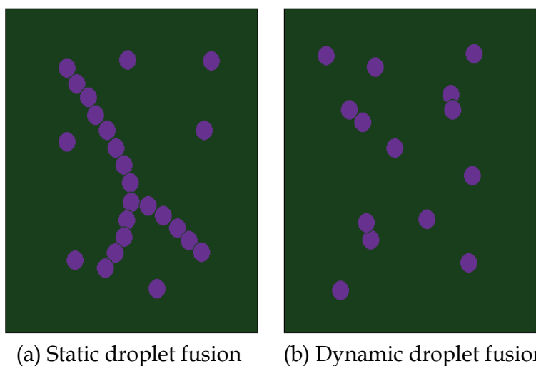
Fig. 6. Dynamics of droplet fusion
