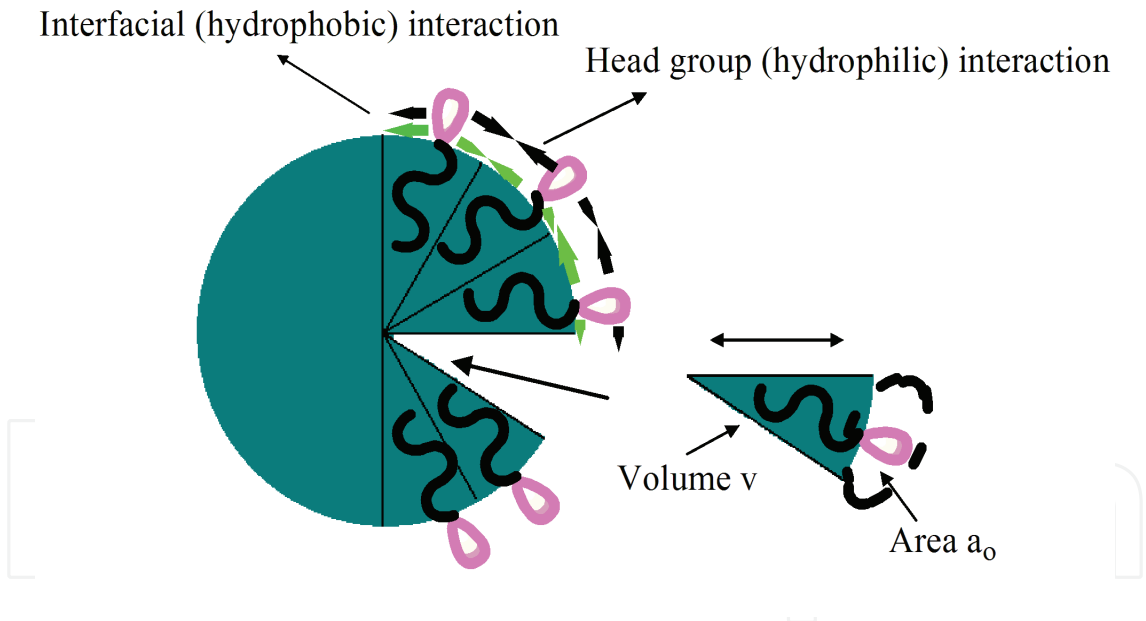
Fig. 3. The critical packing parameter relates the head group area, the length and the volume of the carbon chain into dimensionless number (eqn. 1)
