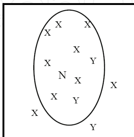
Fig. 2. Graphical representation of k-NN classification (Two Crows, 1999)
