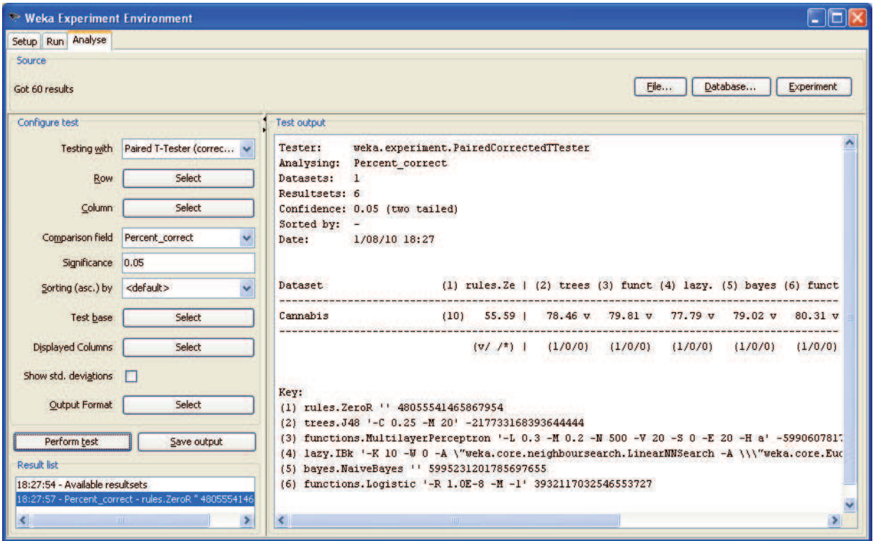
Fig. 9. Comparison of the accuracy (percent correct) between techniques
