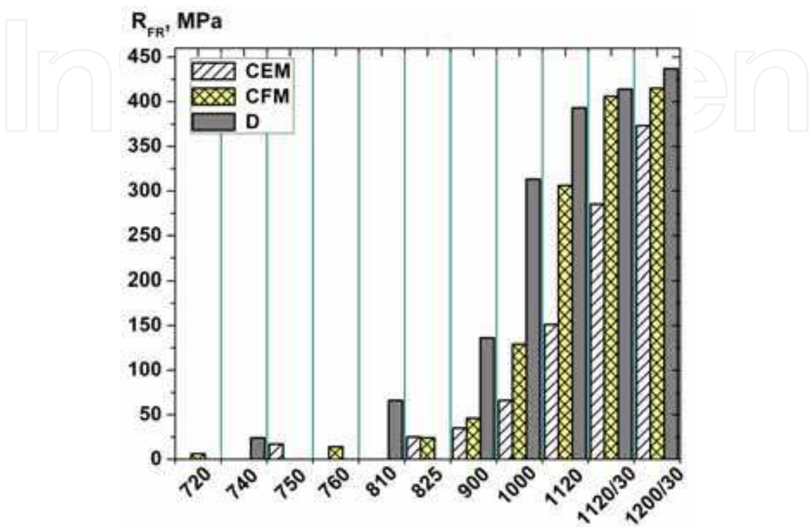
Fig. 24. Rupture strength of interrupted sintered specimens of Fe-0.8Mn-0.5C material, based on admixed with electrolytic manganese (CEM) and ferromanganese (CFM) systems as well as fully prealloyed powder (D), (Hryha et al., 2010-b)
