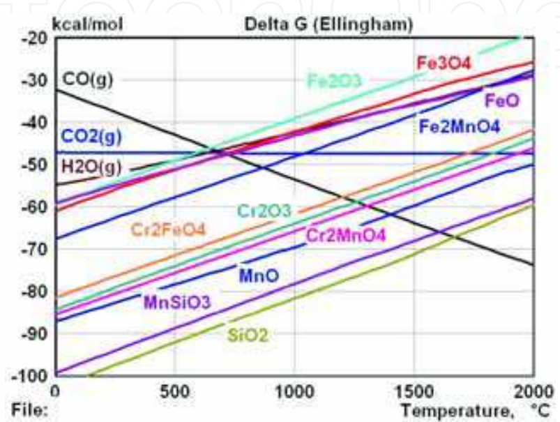
Fig. 2. Ellingham-Richardson diagram indicating stability of oxides
