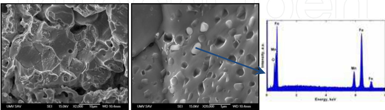
Fig. 20. SEM+EDX analysis of particulate inclusions on the inter-granular decohesion facets around ferromanganese residue after sintering at 1120°C for 30 min on the fracture surface of Fe-0.8Mn-0.5C material
