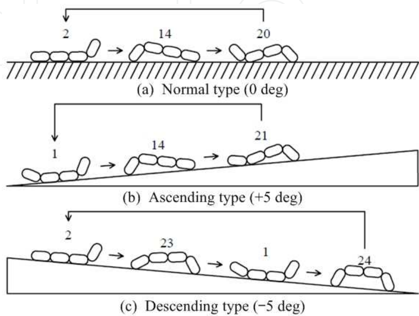
Fig. 10. Optimal motion forms in the three environments
