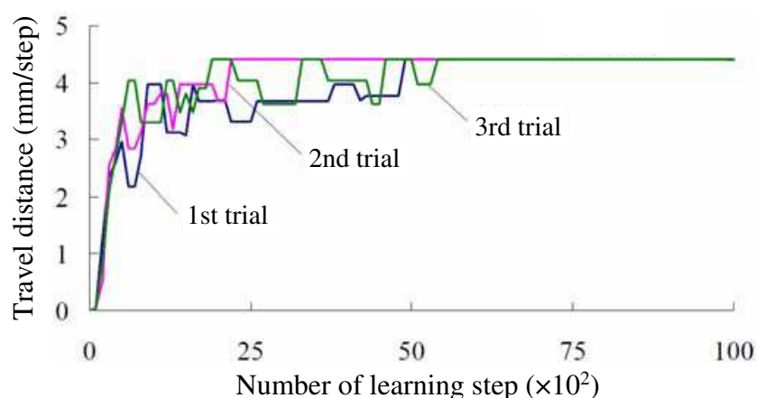
Fig. 6. Relationships between the number of learning step and averaged distance traveled by the caterpillar-shaped robot in a step under Q-learning conditions \alpha = 0.9 and \gamma = 0.8
