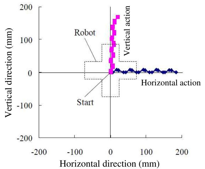
Fig. 15. Trajectories of the starfish-shaped robot in the horizontal and vertical directions This difference would come from the availability of side legs (right and left motors); without the side legs, it can be considered that Q-learning of the starfish-shaped robot is almost the same as that of the caterpillar-shaped robot. Focusing on the motion form, it should be noted that the front and rear motors are driven for the advancement motion, whereas the right and left motors are used for helping the advancement motion. That is, it is thought that the motions of side legs prevent the starfish-shaped robot from slipping on the flat floor or moving backward. In fact, if the optimal motion form is performed without side legs, the travel distance in one step becomes significantly short. Therefore, these results imply that the starfish-shaped robot skillfully employed the advantage of the swing legs.
