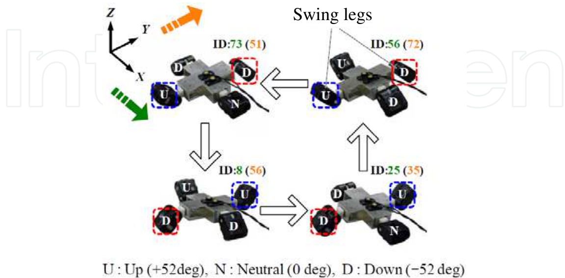
Fig. 13. Optimal motion form for the advancement motion in the X direction
