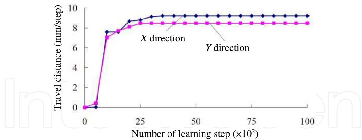
Fig. 14. Relationships between the number of learning step and averaged distance traveled by the starfish-shaped robot per a step under Q-learning conditions \alpha = 0.9 and \gamma = 0.9
