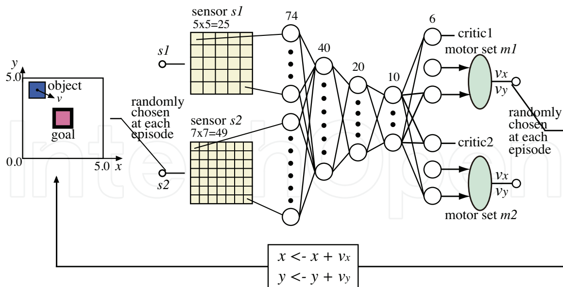
Fig. 11. Abstraction task. One of the two sensors and one of the two motor sets are randomly chosen at each episode. Learning is done for 3 of 4 combinations and the performance of s2-m2 combination is observed.
