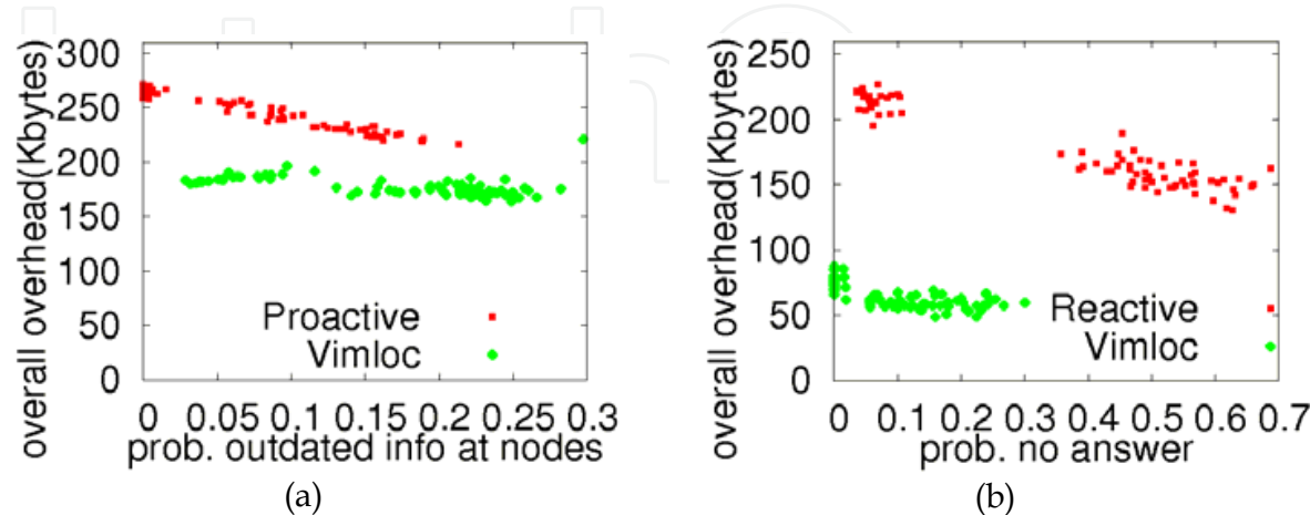
Fig. 9. (a) OO vs. probability of outdated info at nodes (update procedure) and (b) OO vs. probability of no answer (request-reply procedure)
