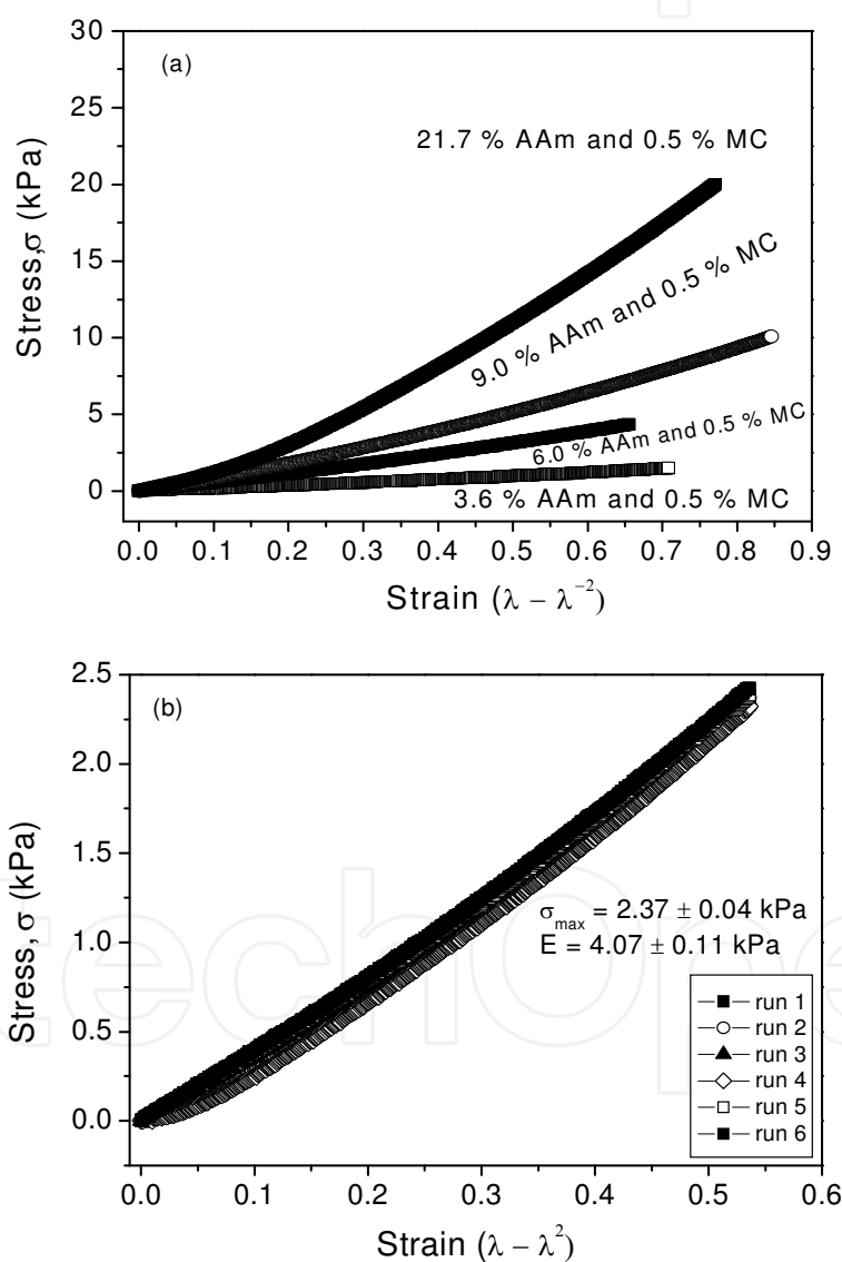
Fig. 3. Measured force and stress as a function of Strain ( \lambda - \lambda^{-2} ) at 25 °C for hydrogels synthesized with (a) [MC] = 0.5 in w:v%, [MBAAm] = 8.6 \mu\text{mol mL}^{-1} and different AAm concentrations; (b) [AAm] = 6.0 in w:v%, [MBAAm] = 10.0 \mu\text{mol mL}^{-1} , [MC] = 0.75 in w:v% [Aouada et al., 2009b].
