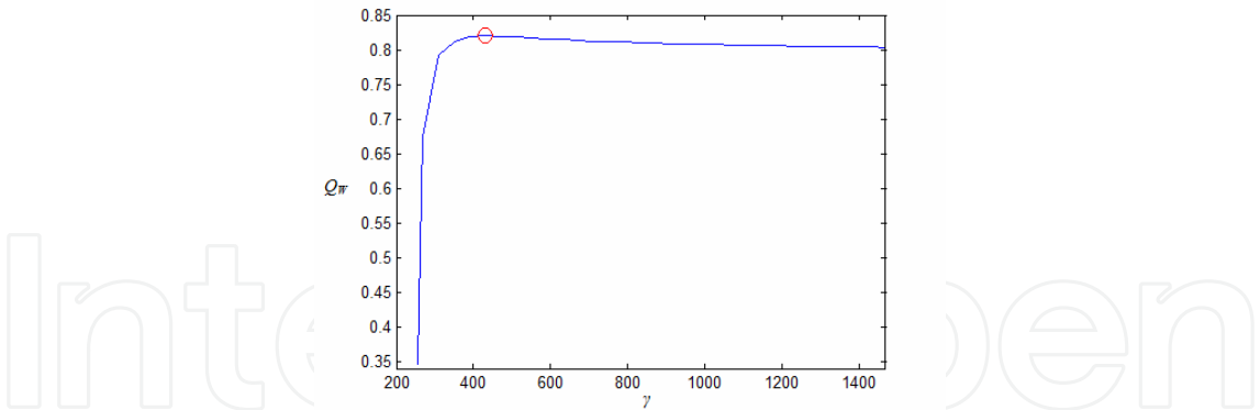
Fig. 11. Plot of Q_W vs. \gamma for image fusion results in Figure 9, indicating a maximum at \gamma = 430 , Q_W = 0.8200
