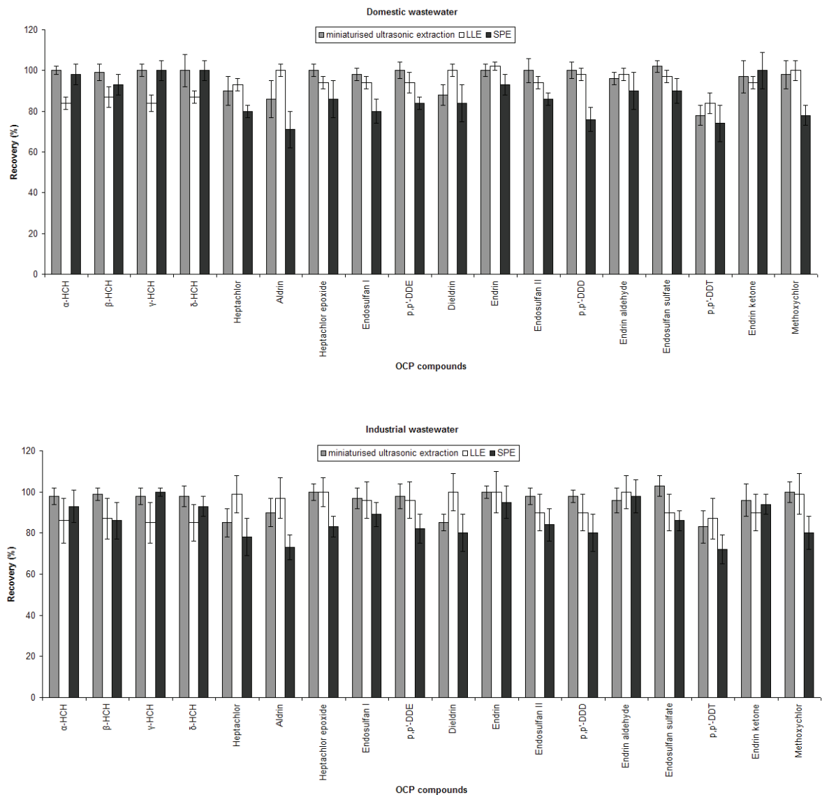
Fig. 3. Comparison of extraction efficiency of the miniaturised ultrasonic extraction method with LLE and SPE for OCPs in fortified real wastewater (domestic and industrial) samples (fortification concentration for each compound: 2 \mu\text{g L}^{-1} ), [n=4] .
