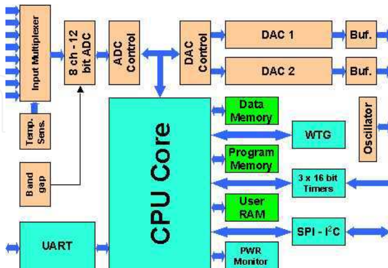
Fig. 5. Block diagram of the ADuC812 Microcontroller.
