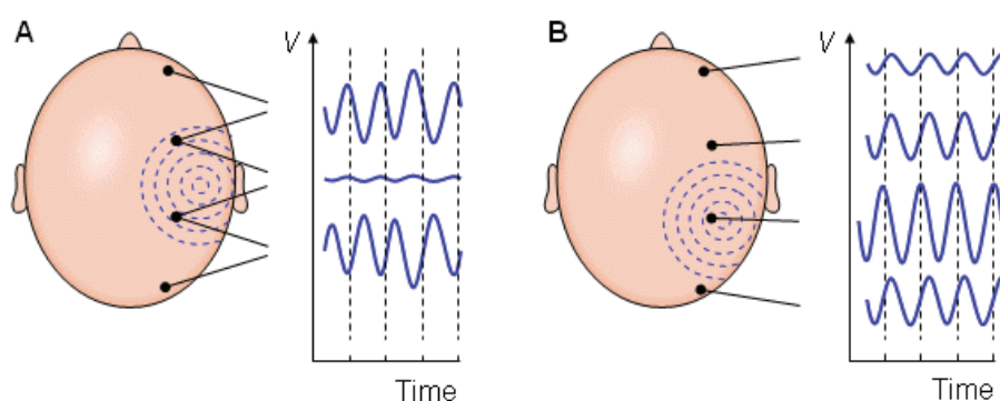
Fig. 2. EEG signal differences presented when a bipolar (A) and unipolar or referential (B) montage is used. In the bipolar montage the signal is a result of potential difference between pairs of electrodes while for the unipolar montage the signal is obtained by the difference in potential between an electrode and a reference point (equal for the whole montage)
