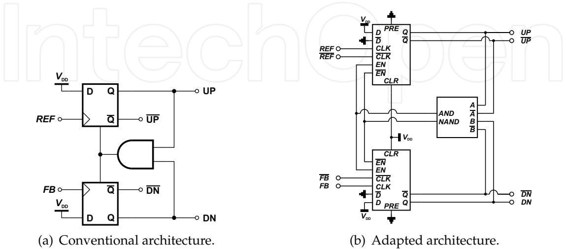
Fig. 25. Phase/frequency detector.
