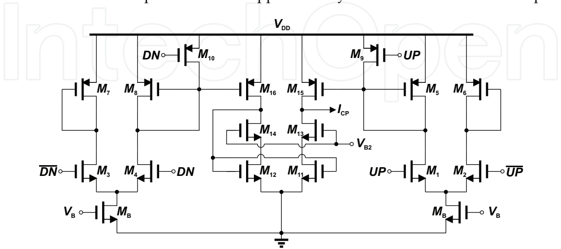
Fig. 26. Current-steering charge pump.
