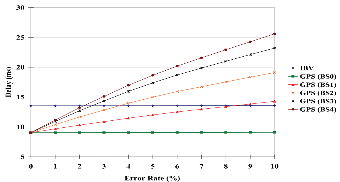
Fig. 9. Delay vs. error rate
