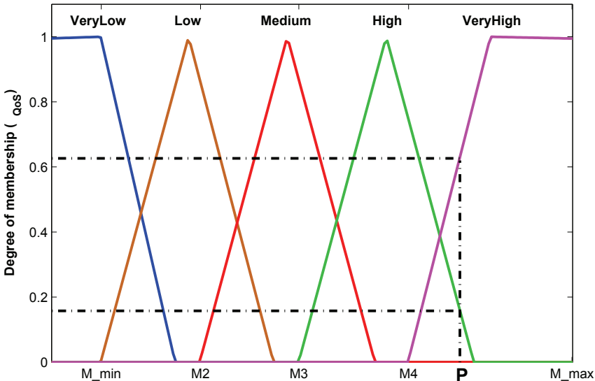
Fig. 4. Membership function
