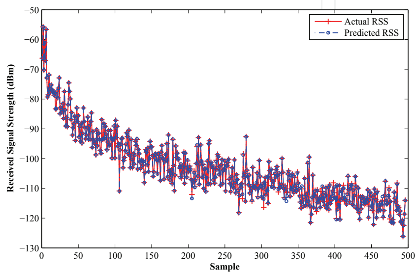
Fig. 3. Prediction results by using back-propagation neural network
