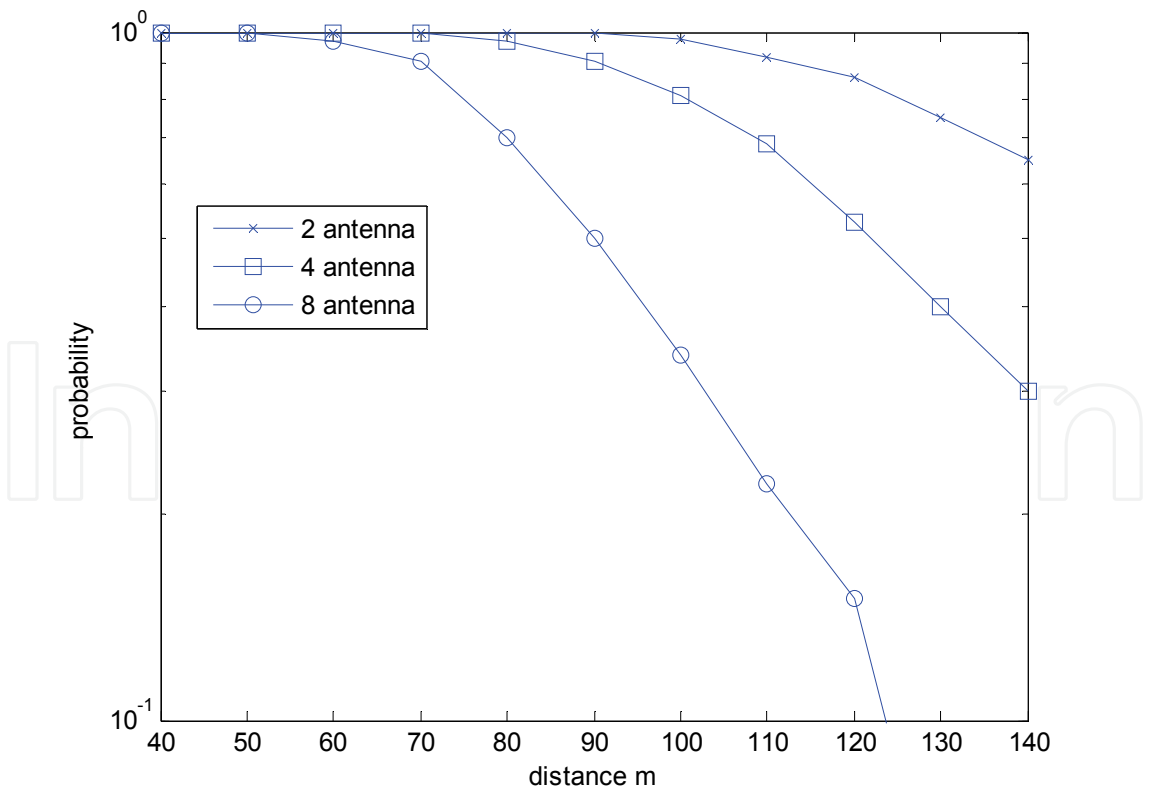
Fig. 14. Probability of correct receiving a data packet by varying the distance and number of transmitter antennas
