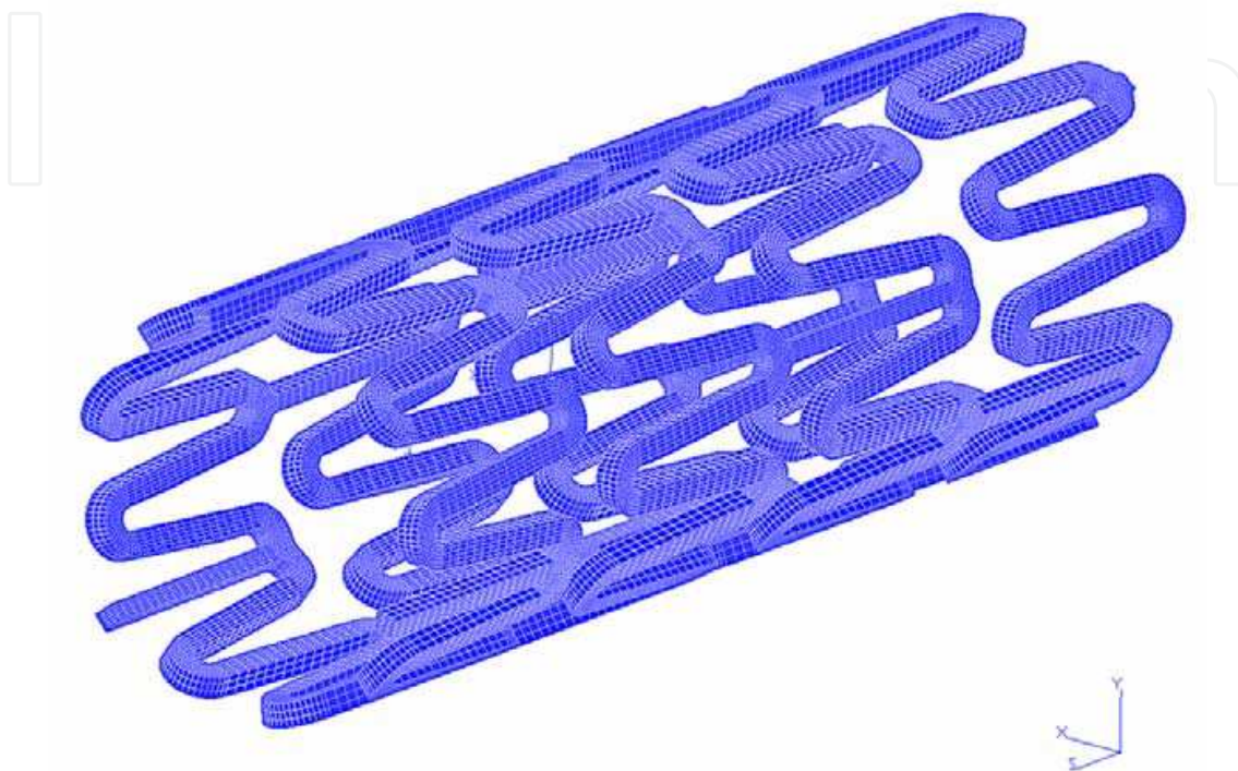
Fig. 9. A 6x3 mesh stent finite element model for combined cardiac pulsatile fatigue and respiratory bending fatigue
