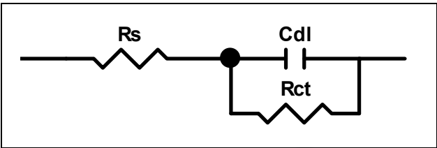
Fig. 3. Equivalent Electric Circuit (Randless) of the electrode-electrolyte interface. The impedance value of the system represented in Fig. 3 is shown in equation (16):
