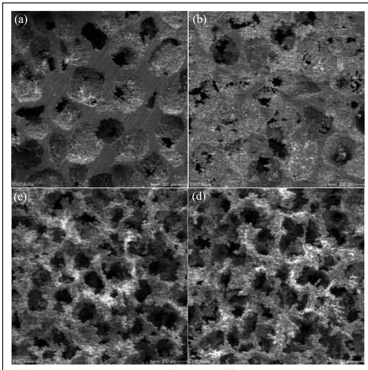
Fig. 10. SEM micrographs of the Ti foams with the same pore size of 250 \mu\text{m} but different porosities of 30 % (a), 45% (b), 55% (c) and 70% (d). Scale bars, 300 \mu\text{m} .
