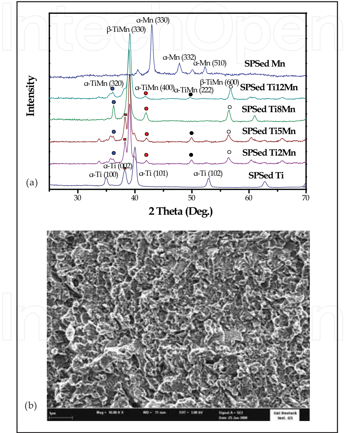
Fig. 4. XRD patterns of the spark plasma sintered Ti, Mn and TiMn alloys showing the TiMn alloys are \alpha+\beta phase alloy (a) and SEM micrograph of the fracture surface of a Ti8Mn alloy.
