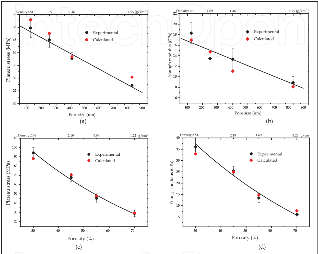
Fig. 11. The effects of pore sizes (a, b) and porosities (c, d) on the plateau stress and Young's modulus of the Ti foams.
