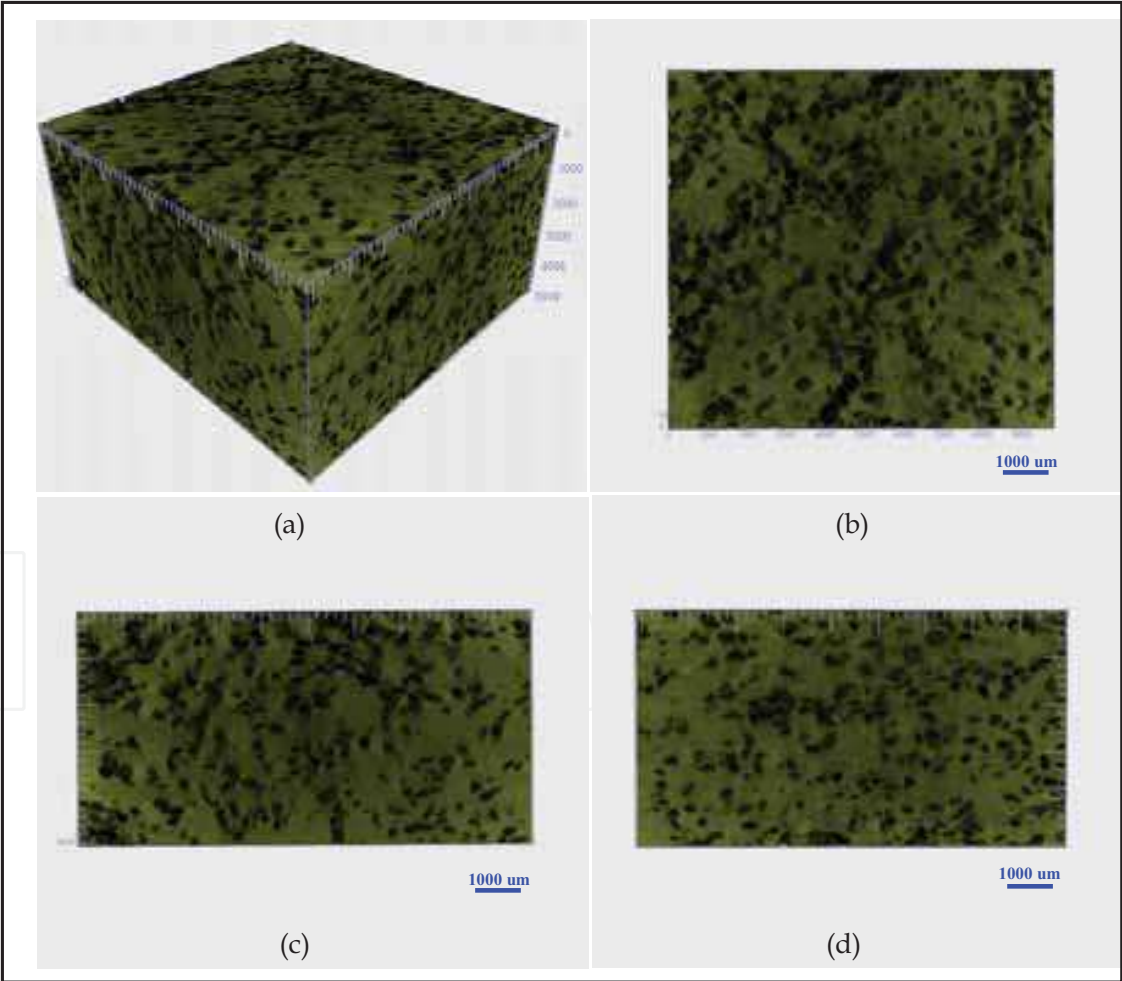
Fig. 7. Micro-CT 3D reconstructions of the Ti foam with \text{NH}_4\text{HCO}_3 and \text{TiH}_2 as pore forming agents produced at 1000^\circ\text{C} by free pressureless SPS method with an isometric view (a), 2D top view (b), left side view (c), and right side view (d). Scale spacing, 1000 \mu\text{m} .
