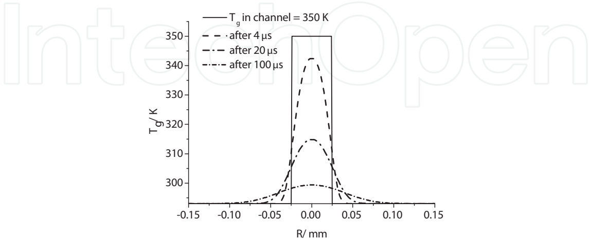
Fig. 8. Spatial distribution of the gas temperature (radially along the electrode) in the afterglow phase in the gap between electrodes for Al-spike as the opposite electrode.
