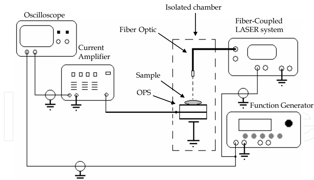
Fig. 11. Experimental setup for opacity measure
