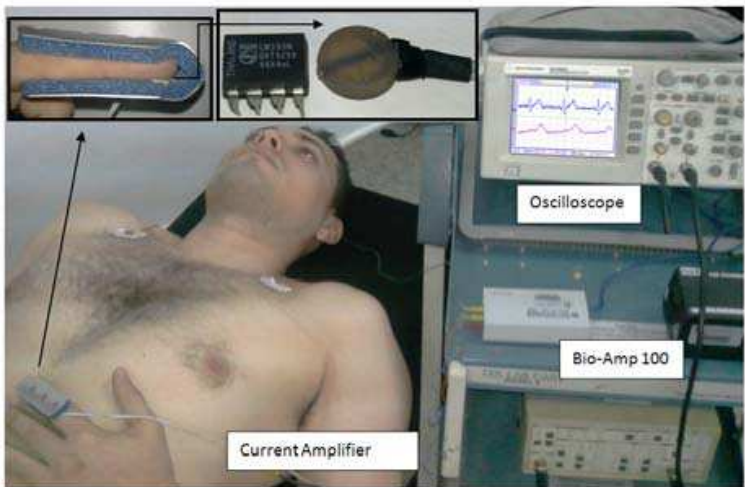
Fig. 8. Real setup used for get fingertip pulses
