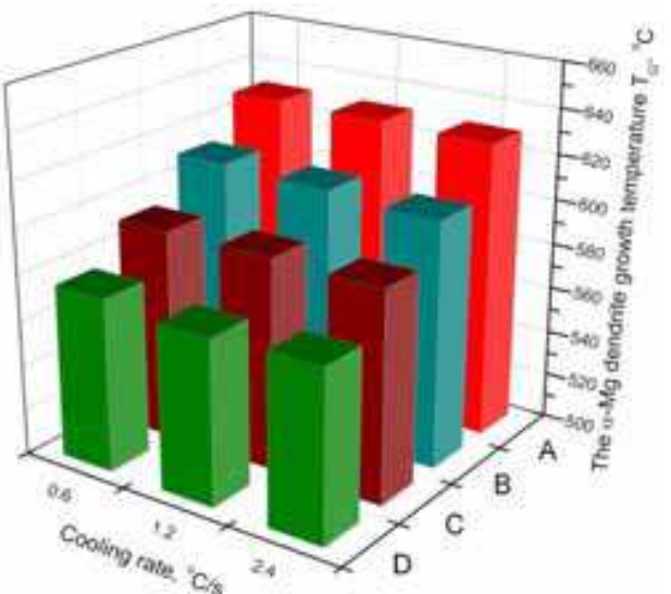
Fig. 18. Influence of cooling rate on Mg dendrite growth temperature ( T_G ): A - MCMgAl3Zn1, B - MCMgAl6Zn1, C - MCMgAl9Zn1, D - MCMgAl12Zn1
