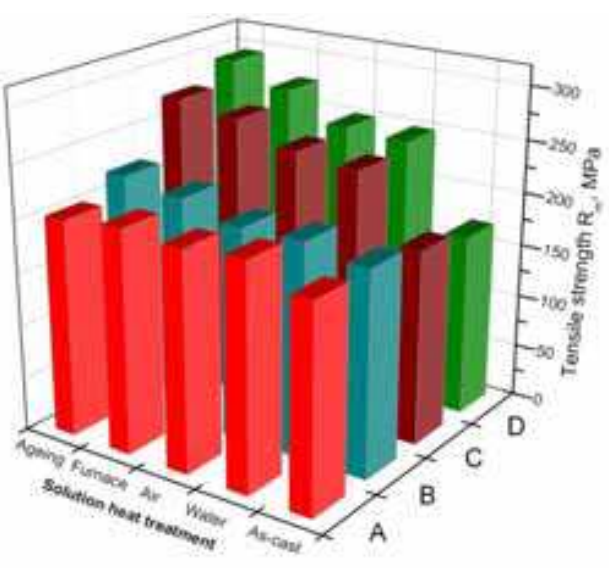
Fig. 13. Results of tensile strength Rm measurements of magnesium cast alloys: A - MCMgAl3Zn1, B - MCMgAl6Zn1, C - MCMgAl9Zn1, D - MCMgAl12Zn1
