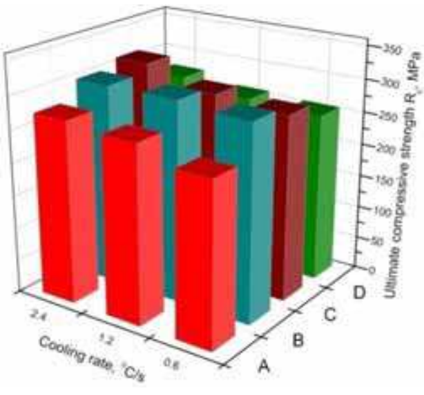
Fig. 22. Influence of cooling rate on ultimate compressive strength Rc: A – MCMgAl3Zn1, B – MCMgAl6Zn1, C – MCMgAl9Zn1, D – MCMgAl12Zn1
