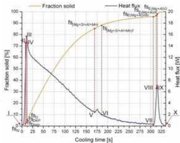
Fig. 16. Representative curves illustrate changes of heat flux and fraction solid of MCMgAl6Zn1 alloy MCMgAl6Zn1 cooled at 0.6°C/s
