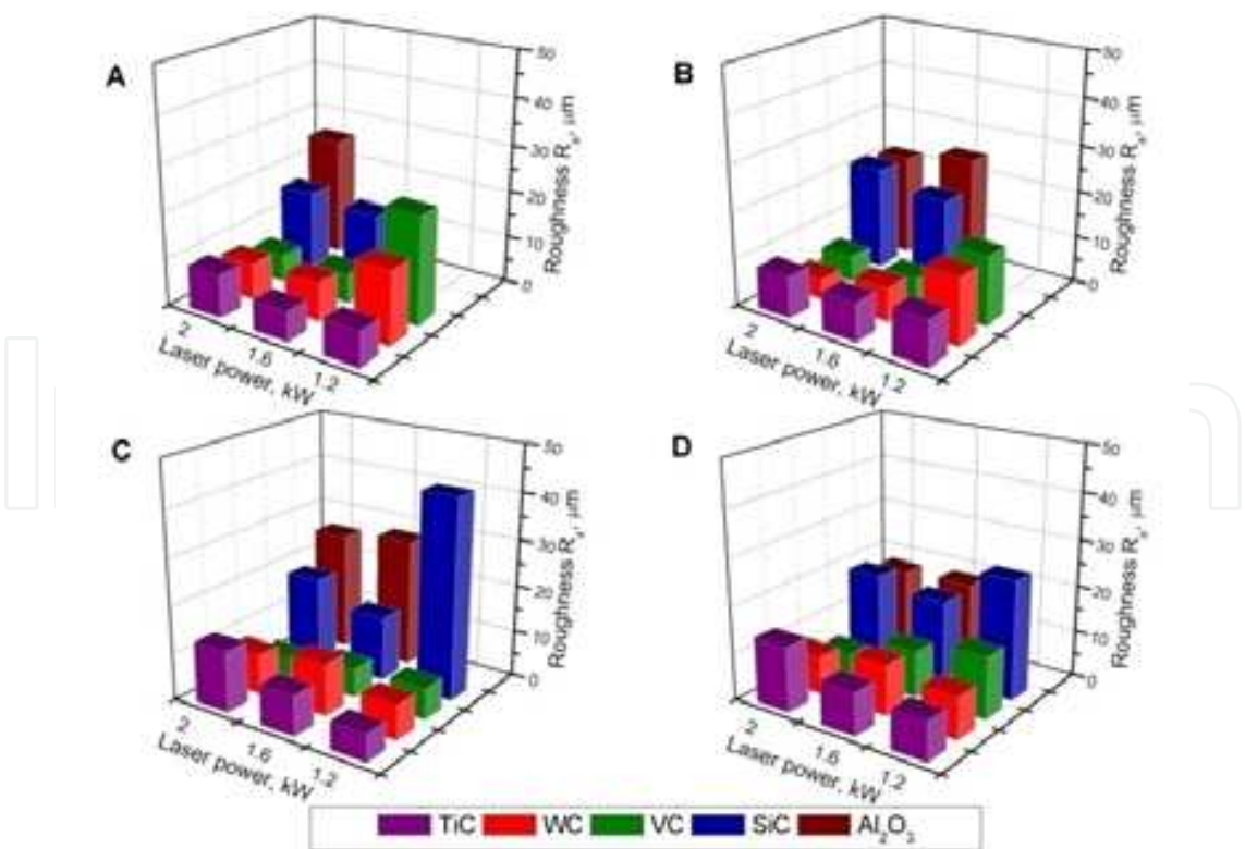
Fig. 24. Laser power and Al mass concentration influence on roughness of alloyed surface layer: A – MCMgAl3Zn1; B – MCMgAl6Zn1 ; C – MCMgAl9Zn1; D – MCMgAl12Zn1
