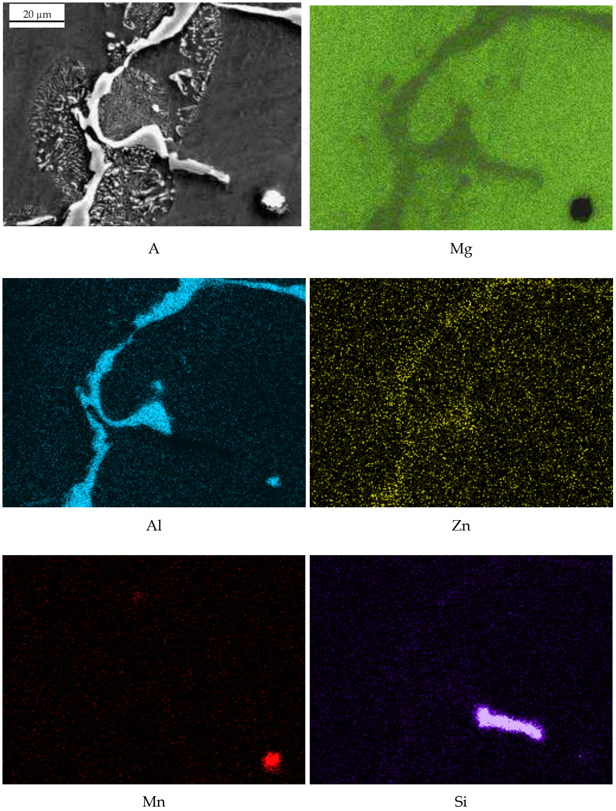
Fig. 7. The area analysis of chemical elements alloy MCMgAl6Zn1 after cooling in the furnace: image of secondary electrons (A) and maps of elements' distribution
