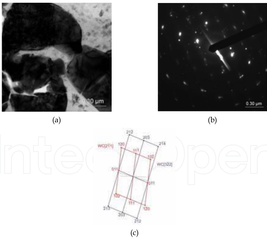
Fig. 30. TEM image of the surface layer of MCMgAl9Zn1 alloy after alloying with WC: a) bright field; b) diffraction pattern of area shown in a), c) part of solution for diffraction pattern shown in b
