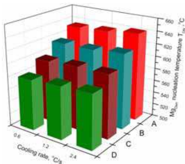
Fig. 17. Influence of cooling rate on Mg_{Den} nucleation temperature ( T_{DN} ): A - MCMgAl3Zn1, B - MCMgAl6Zn1, C - MCMgAl9Zn1, D - MCMgAl12Zn1
