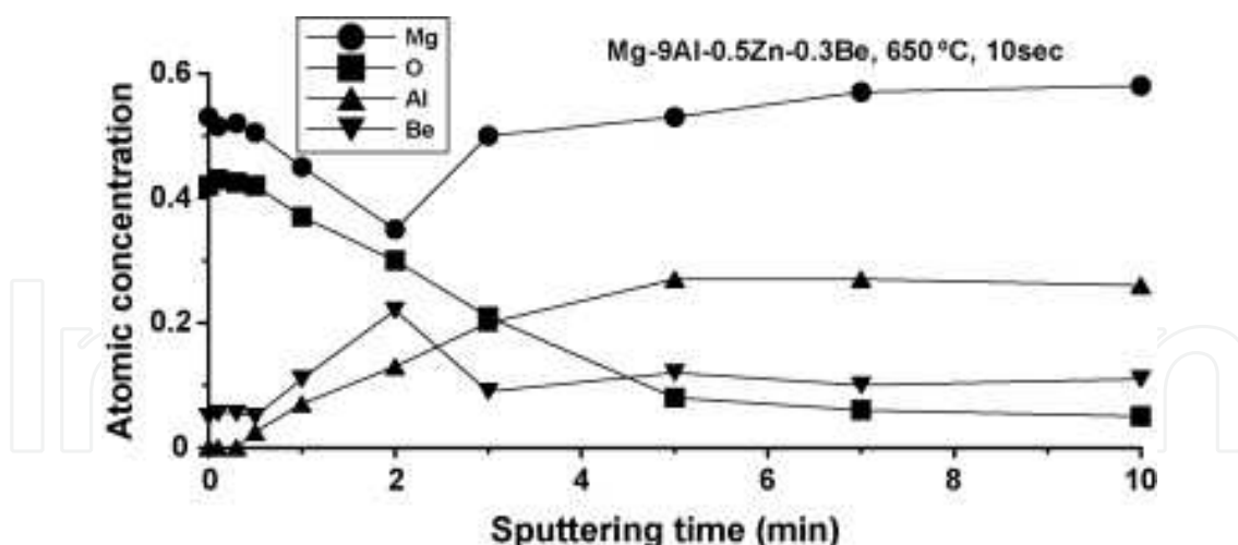
Fig. 10. Relation of Al, O, Mg and Be concentrations versus sputtering time for sample of AZB91 alloy melted at 923 K for 10 s
