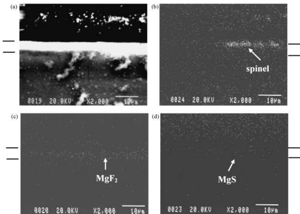
Fig. 4. EPMA photos showing the sectional view including oxide film and substrate; sample (99.956 wt.% Mg) heated in a protective atmosphere (0.2% \text{SF}_6 ) at 700 K for 25 h; sample polished by abrasive papers; (a) magnification 2000 \times ; (b) Al mapping; (c) F mapping and (d) S mapping.
