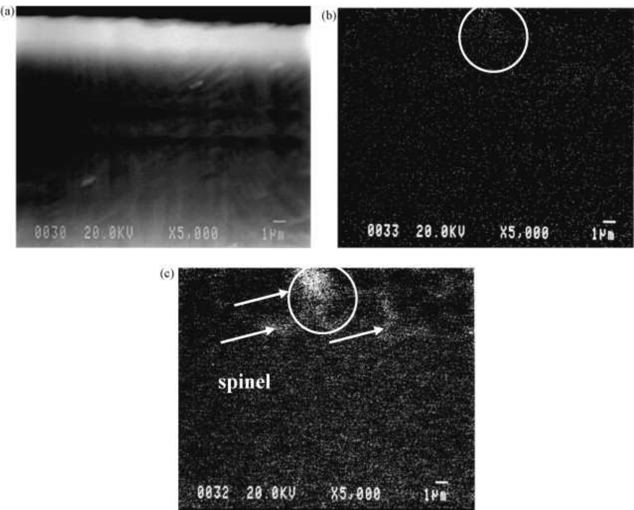
Fig. 8. EPMA photos showing the sectional view including oxide film and substrate; solution-treated AZ80 heated in air at 700 K for 1 h; sample polished by abrasive papers; (a) magnification 5000×; (b) O mapping and (c) Al mapping.
