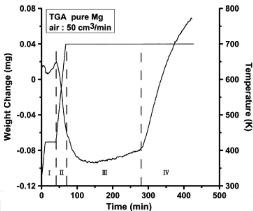
Fig. 1. Thermogravimetric analysis of pure magnesium (99.96 wt.%); heating rate \partial T / \partial t = 10 °C min -1 ; air flowing rate = 50 cm 3 /min.
