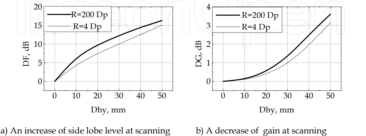
Fig. 16. Changes of antenna parameters at scanning.
