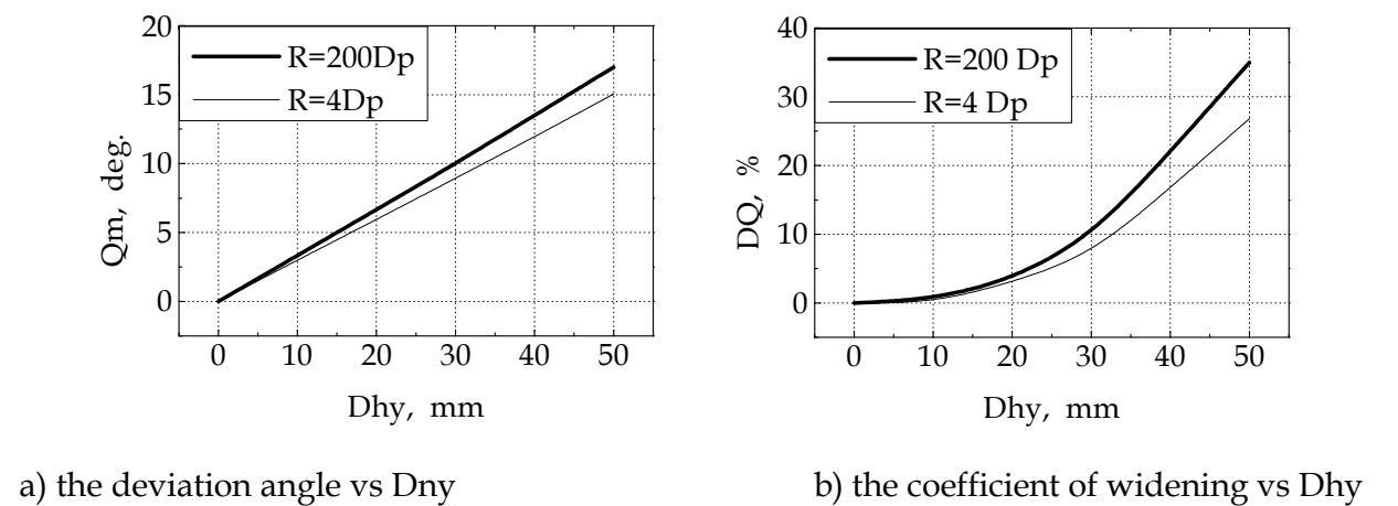
Fig. 15. Scanning in a reflector antenna.
