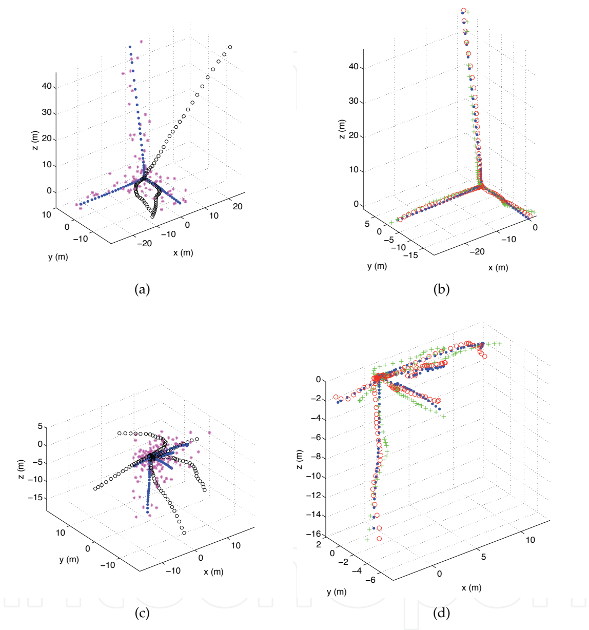
Fig. 5. Blue points represent true MAVs trajectories, black circles are the trajectories with only odometric estimates, magenta stars are the GPS data, green stars are the trajectory estimates without taking into account relative observations and red circles are the estimates with the complete distributed EIF. Figures 5(a)-5(b) are the simulation of 3-MAV scenario, while in Figures 5(c)-5(d) is plotted the evolution of a 5-MAV system.
