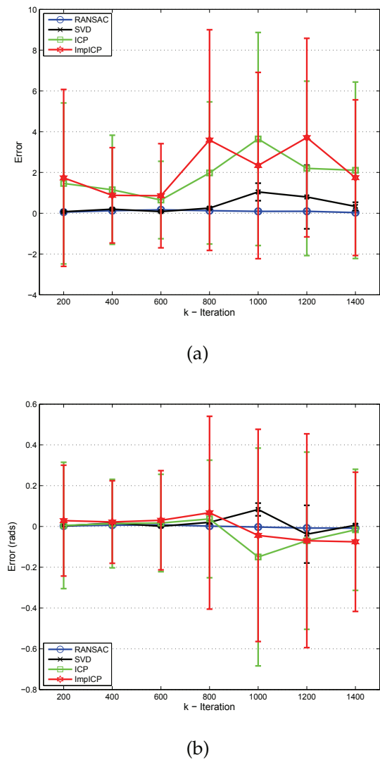
Fig. 2. (a) Traslation error. (b) Rotation error.
