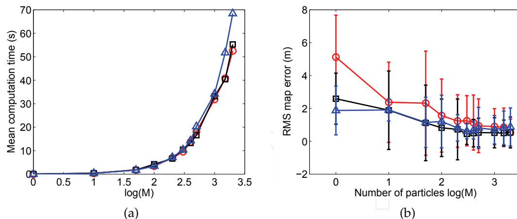
Fig. 6. Figure (a) shows the mean computation time at each iteration of the algorithm for different number of particles M = \{1 \ 10 \ 50 \ 100 \ 200 \ 300 \ 400 \ 500 \ 1000 \ 1500 \ 2000\} . Figure (b) shows the RMS error in the map when B/K observations are used. We show simultaneously results with one robot ( \circ ), two robots ( \square ) and three robots ( \triangle ).
