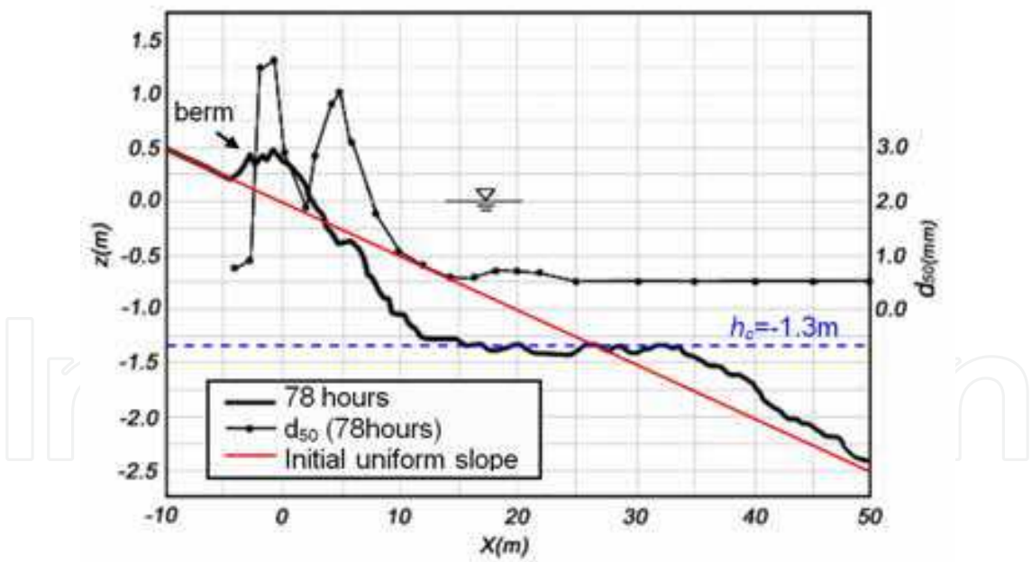
Fig. 3. Change in longitudinal profile and cross-shore distribution of d_{50} in experiment using large wave tank (Meguro et al., 2005)
