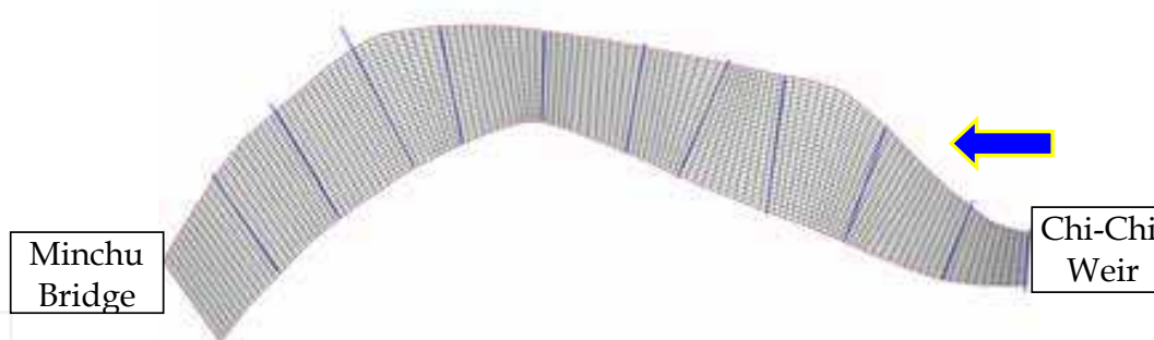
Fig. 15. Computational mesh in the channel downstream of the Chi-Chi Weir
