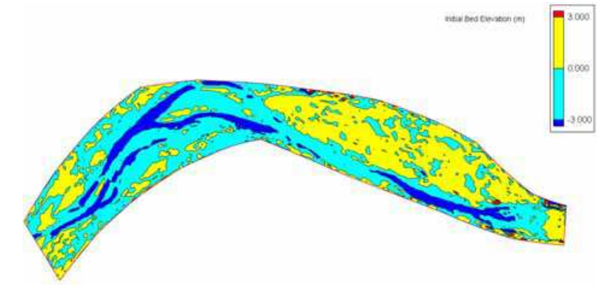
Fig. 3. Scouring and deposition pattern in the downstream channel of the Chi-Chi Weir (2004-2007)
