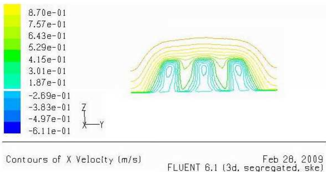
Fig. 2. Velocity distribution in y - z plane at x = 0.0 and a Reynolds number is 9.0 \times 10^5
