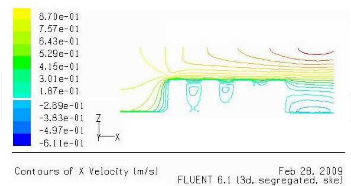
Fig. 7. Velocity distribution in x-z plane at y = 2.0 and a Reynolds number is 9.0 \times 10^5 As shown in Fig. 7, some strong vorticities are found in the every target streets. The first street in the direction of wind has a large vorticity, in the first two streets, there are respectively two vorticities (a large vorticity, a small vorticity), and the vorticity can not be found in the last street. But some vorticities can be found on the lower part of the building in the leeward direction at the bottom of the streets.
