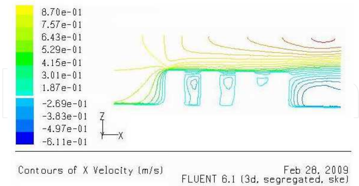
Fig. 5. Velocity distribution in x-z plane at y = 0.0 and a Reynolds number is 9.0 \times 10^5 As shown in Fig. 5, some strong vorticities are found in the every target streets. The flow lines are raised when it first reaches the urban building. The flow lines at roof level are almost parallel to the ground after the flow passed several urban buildings with identical height. The flow under this configuration is found to be stable within the whole simulation period, as also stated by Gerdes and Olivari (1999). [5]
