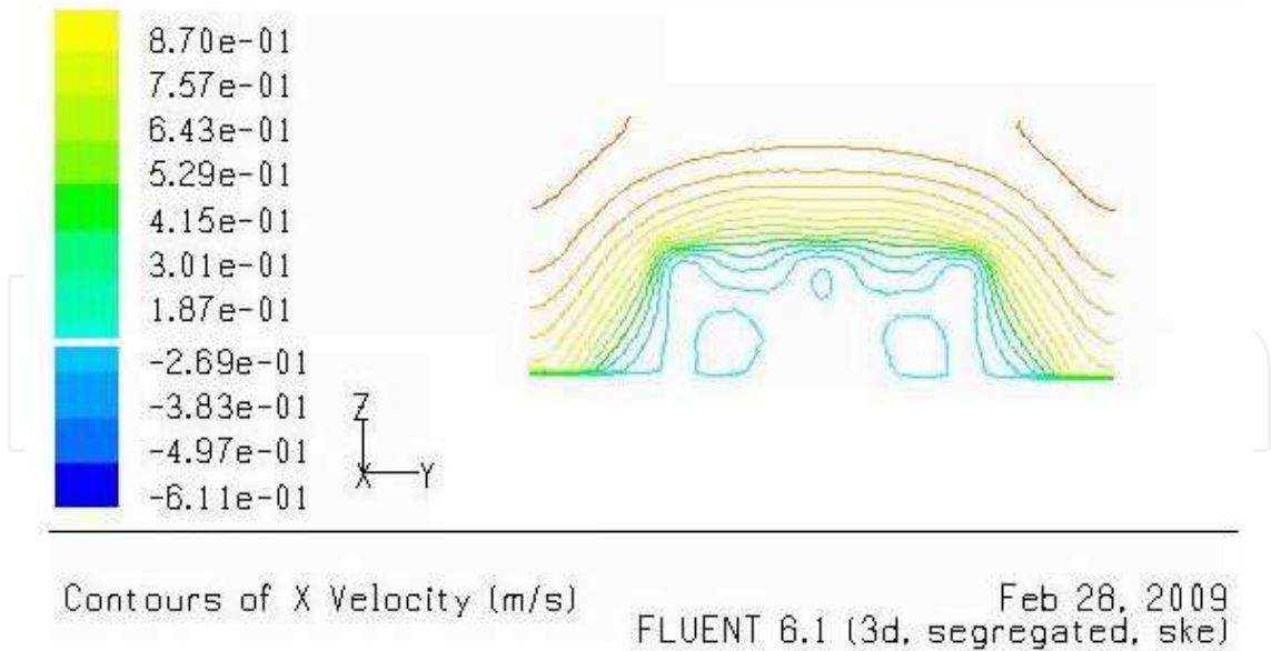
Fig. 4. Velocity distribution in y-z plane at x = 2.0 and a Reynolds number is 9.0 \times 10^5 Fig. 4 depicts clearly some recent circle vorticities in the back of the buildings in the direction of the wind. In the back of the buildings of both sides, a large vorticity is found and in the middle of the back of the building, a vorticity is observed at the top of the streets. In addition, flow lines are basically as the same as the profile of the streets.
