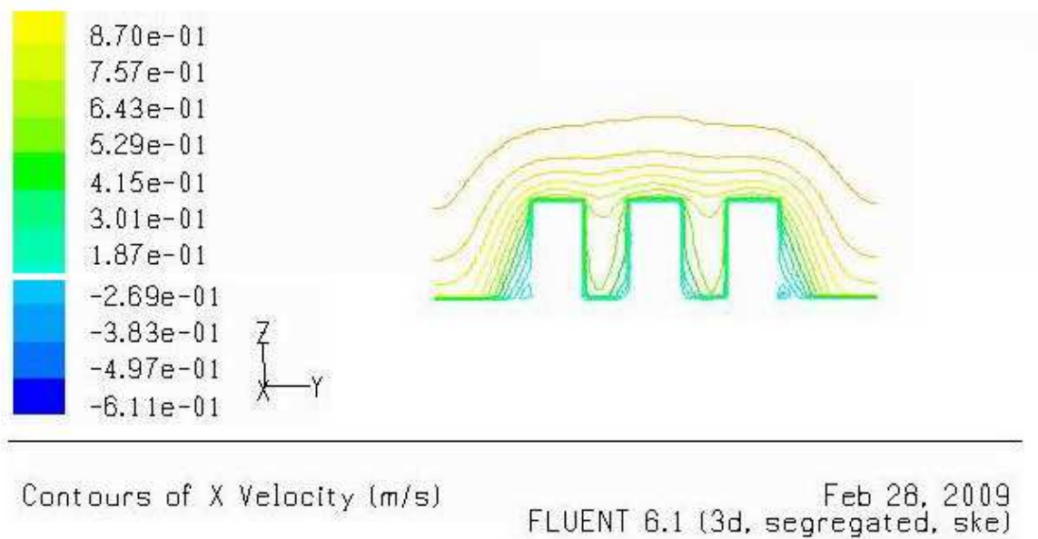
Fig. 3. Velocity distribution in y-z plane at x = 1.0 and a Reynolds number is 9.0 \times 10^5 Fig. 3 shows that in a cross-section of the building, none of vorticity can be found in the streets, but a small vorticity is observed in the bottom of the both sides of buildings. In addition, flow lines are basically as the same as the profile of the streets.
