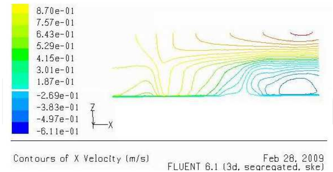
Fig. 6. Velocity distribution in x-z plane at y = 1.0 and a Reynolds number is 9.0 \times 10^5 As shown in Fig. 6, there is no vorticity, in the direction of the wind, the speed lines are sparse, while the flow lines are intensive in the leeward direction, The flow lines at roof level is almost parallel to the ground after the flow passed several urban buildings with identical height.
