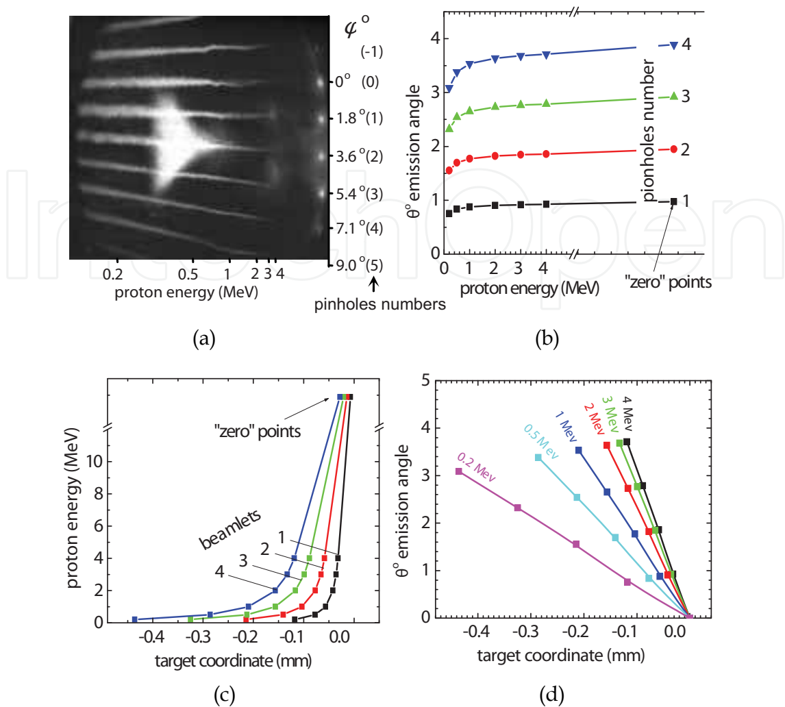
Fig. 16. a) Spectral traces of a row of pinhole images: On the right side of the figure the tilt angle \phi^\circ of the spectral traces from the central symmetry axes corresponding to \phi^\circ = 0 line (target normal) and respective numbers of beam-lets (in brackets) are given. b) Proton emission angle in each beam-let depending on proton energies in beamlets from 1st up to 4th is depicted. c) Emitted proton energy as function of target coordinates in beamlets from 1st up to 4th. d) Emission angle of protons with 0.2, 0.5, 1, 2, 3, and 4 MeV energies dependent on target emission coordinate is exhibited.
