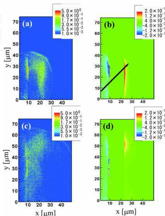
Fig. 10. Temporal evolution of the electron energy density and the longitudinal electric field. The electron energy density is normalized by n_c m_e c^2 , and observed at a) 140 fs, and c) 220 fs. The electric field is normalized by laser electric field, and observed at b) 140 fs, and d) 220 fs. The target width is 13 \mu\text{m} and is located at 10 \mu\text{m} < x < 23 \mu\text{m} . The black line in b) indicates the laser axis.
