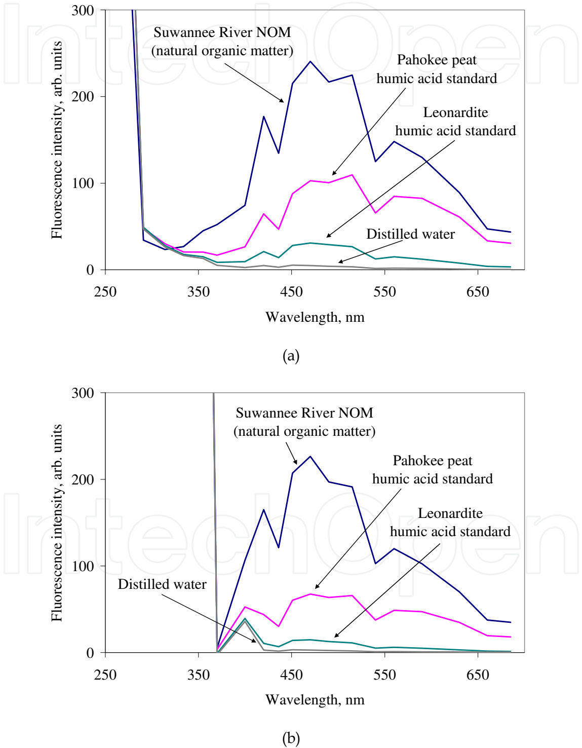
Fig. 13. Fluorescence of humic substances with (a) 266 nm and (b) 355 nm laser excitation
