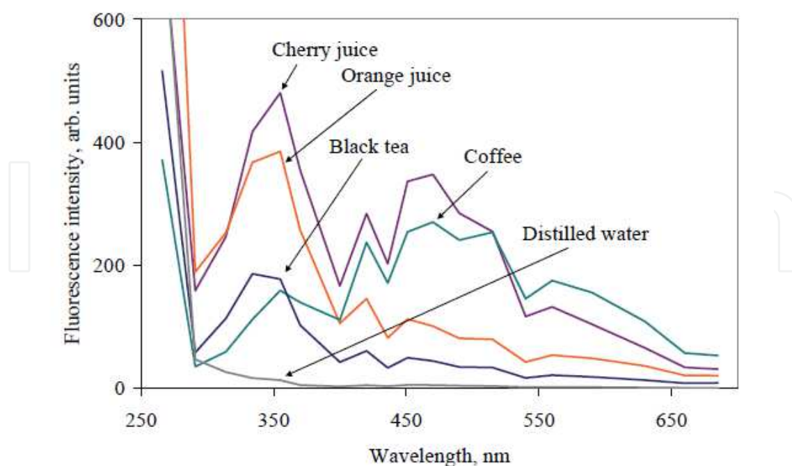
Fig. 12. Fluorescence of various drinks in distilled water; 266 nm laser excitation
