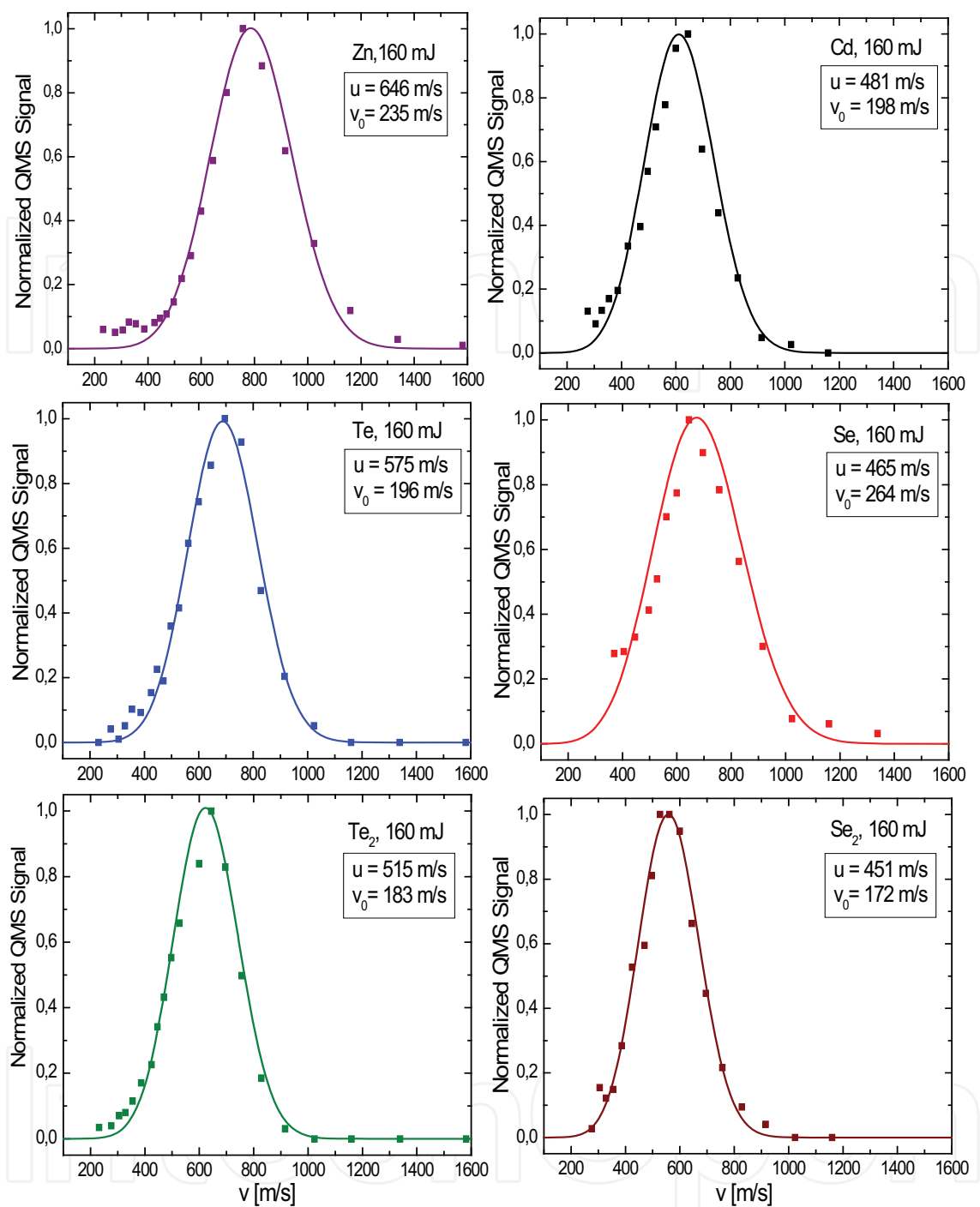
Fig. 13. TOF velocity distributions for CdSe PP and ZnTe PP targets ablated with 160 mJ laser pulses of frequency of 25 Hz Solid curves are obtained from theoretical fit to experimental points with the help of Eq. (7). Fitting parameters u and v_0 are given in the inserts.
