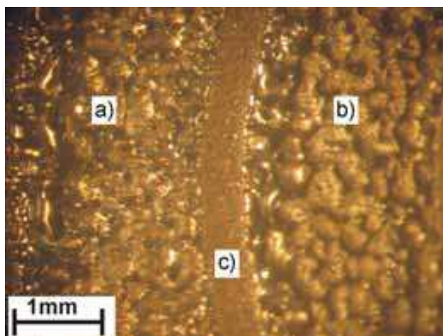
Fig. 4. Surface appearance of CdTe PP target ablated with 160 mJ laser pulses (optical microscope).
