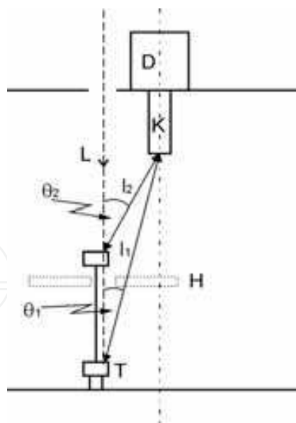
Fig. 2. Sketch of configuration applied for TOF and angular distribution measurements. (D) particle detector (PIC), (K) particle ionizer and quadrupole, (T) target, (L) laser beam, l_1 & l_2 distances between lower and upper position of target, respectively, (H) substrate heater, removed from position for TOF measurements.
