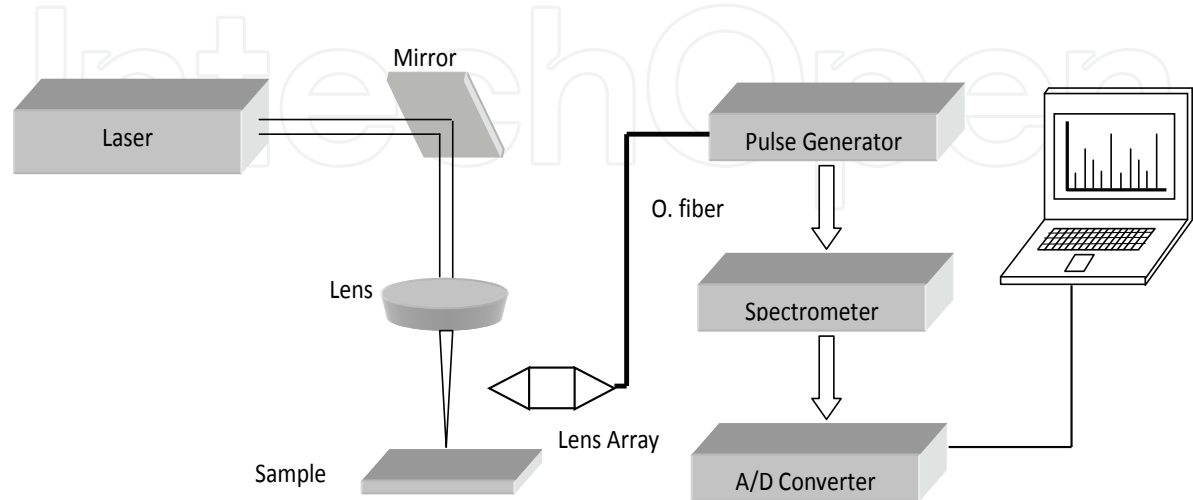
Fig. 1. Schematic of experimental setup For this configuration, the laser can produce a train of pulses with duration for each pulse of about 20 ns, separated by 10 \mu s interval, with a total duration of the pulse train about 700 \mu s. In Figure 2 the acquired signal of laser pulse for passive Q:Switched laser is showed.
