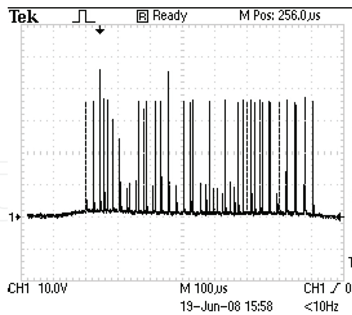
Fig. 2. Oscilogramme of pulse train obtained with passive Q:Switch. All system elements are mounted on a stereo-microscope in order to obtain better facility for positioning and observation of samples as well as to follow the results of irradiation. The dimensions and weight of LIBS device is 40 x 20 x 15 cm and 5 kg respectively. Figure 3 shows a photograph of device, called MicroLIBS.
