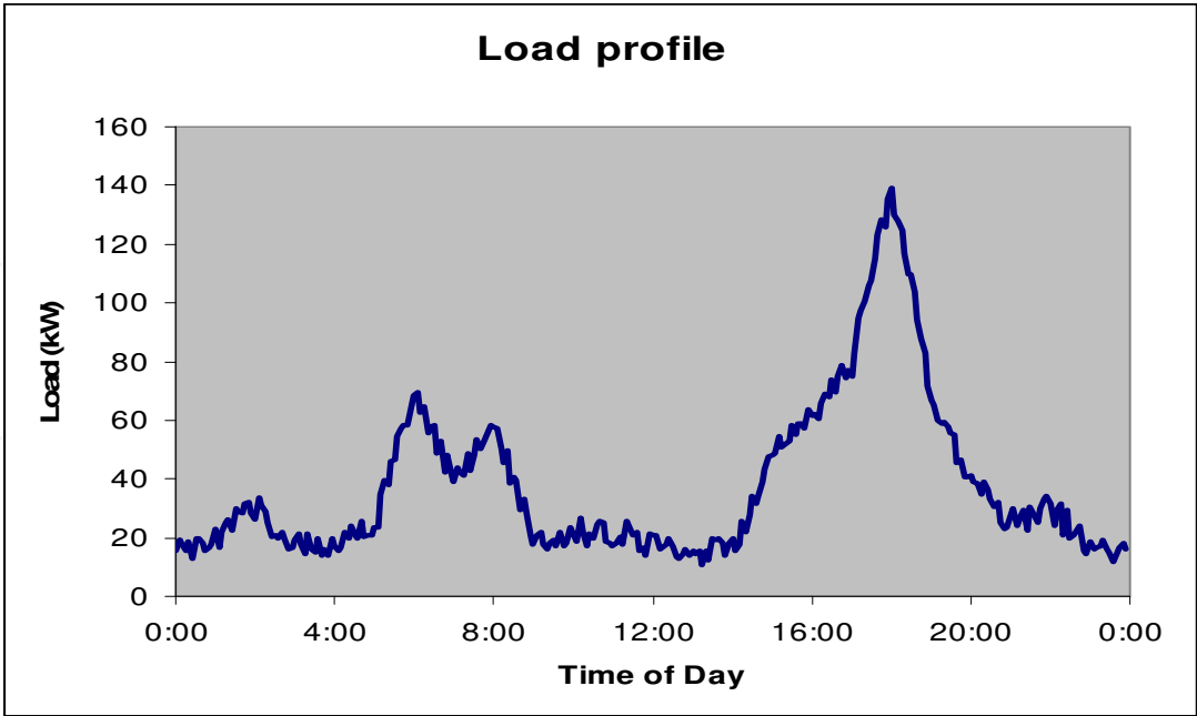
Fig. 1. Typical load profile of a remote community
