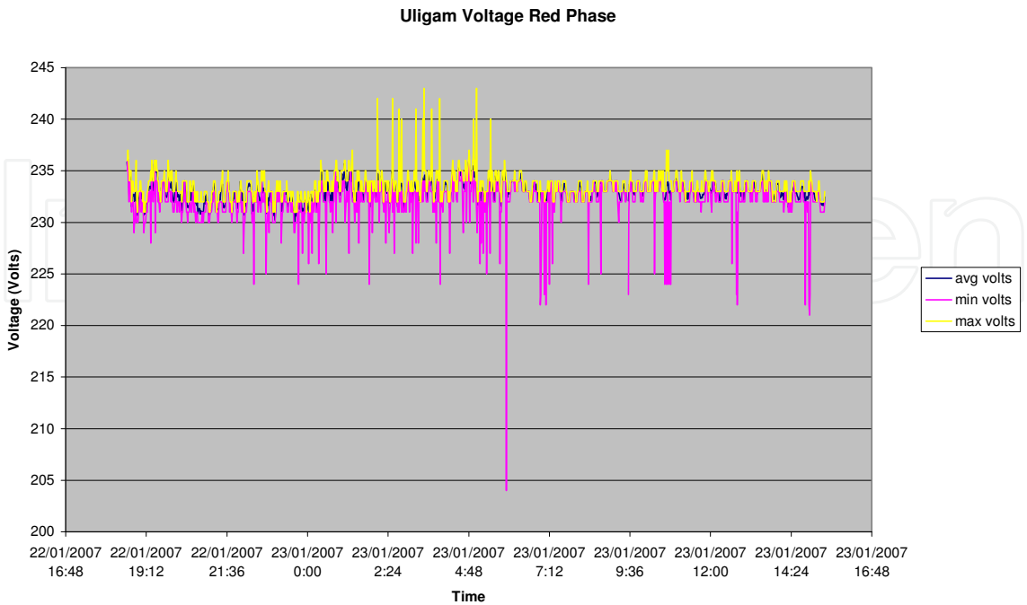
Fig. 9.c- Typical voltage data
