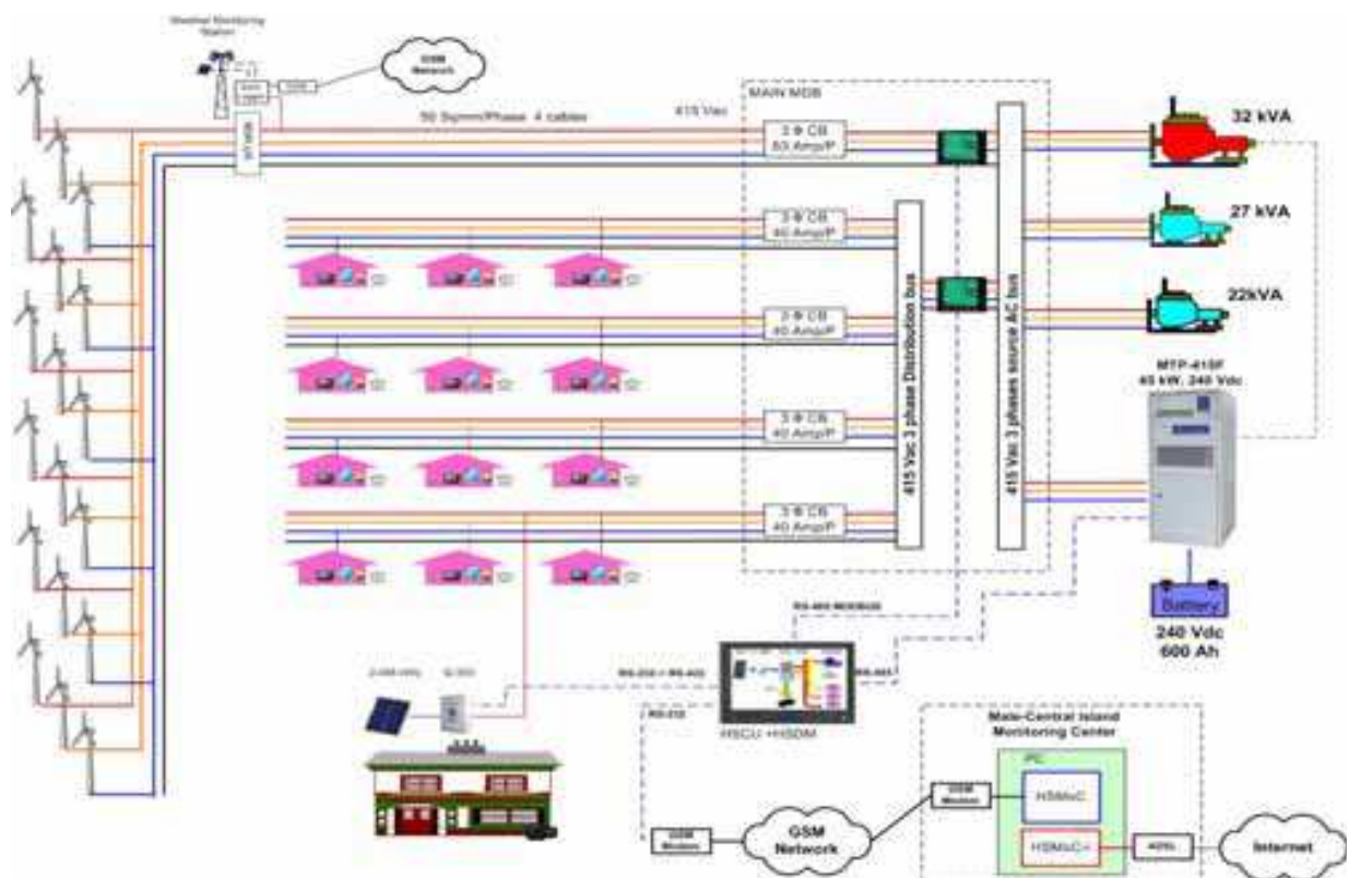
Fig. 11. Typical layout of the hybrid system
