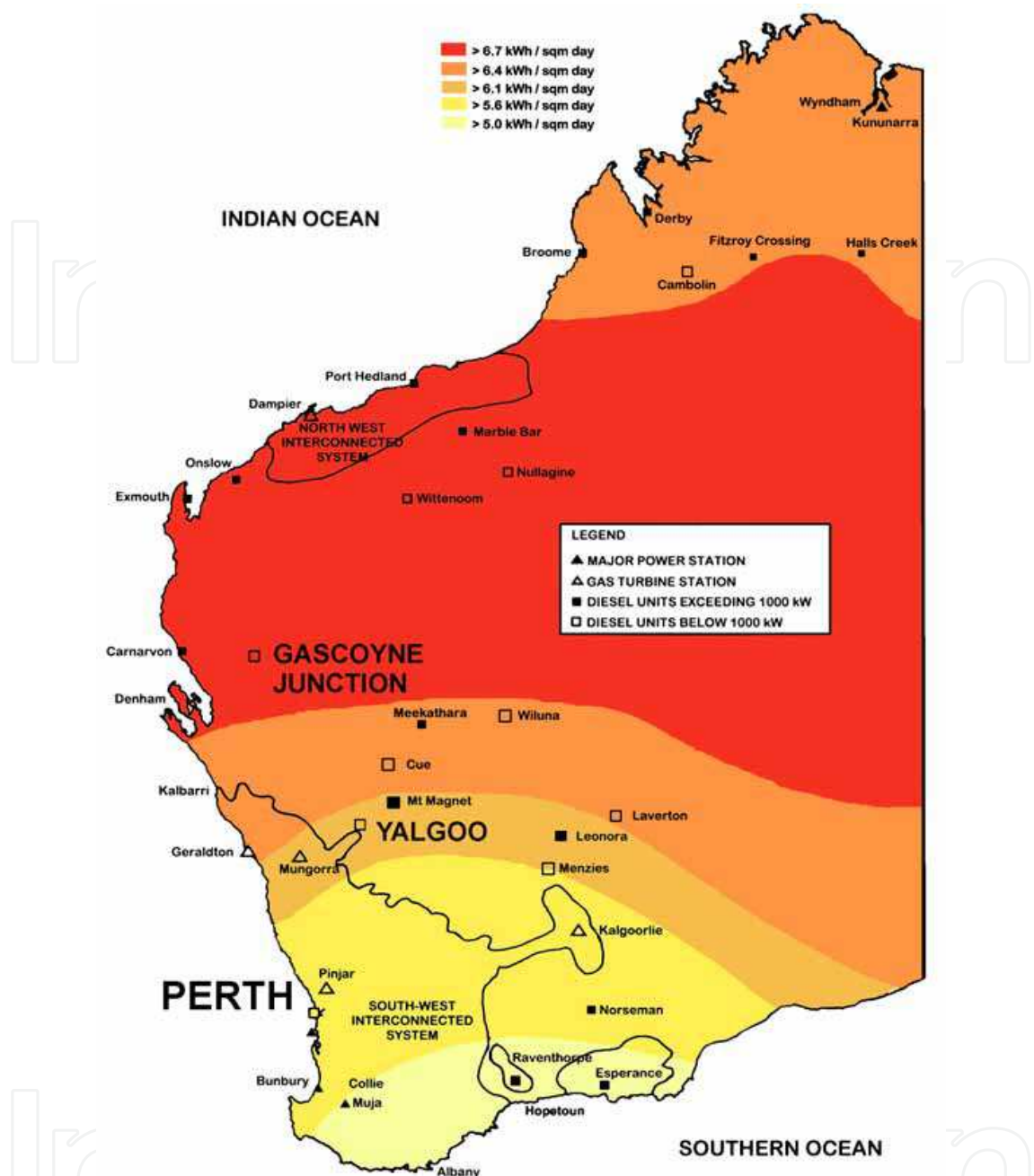
Fig. 17. Annual solar radiation in Western Australia
