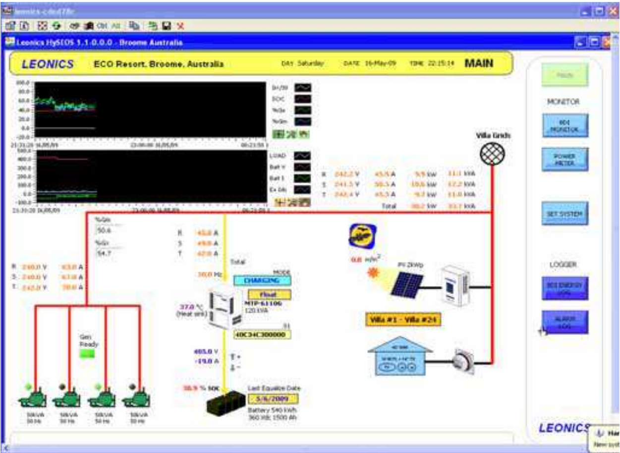
Fig. 20. Remote monitoring display
