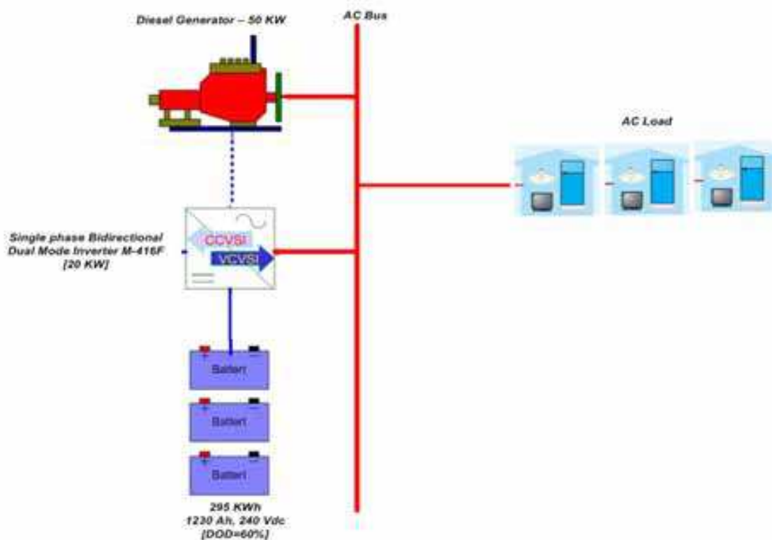
Fig. 3. Battery/ Inverter/ Diesel Generator hybrid system
