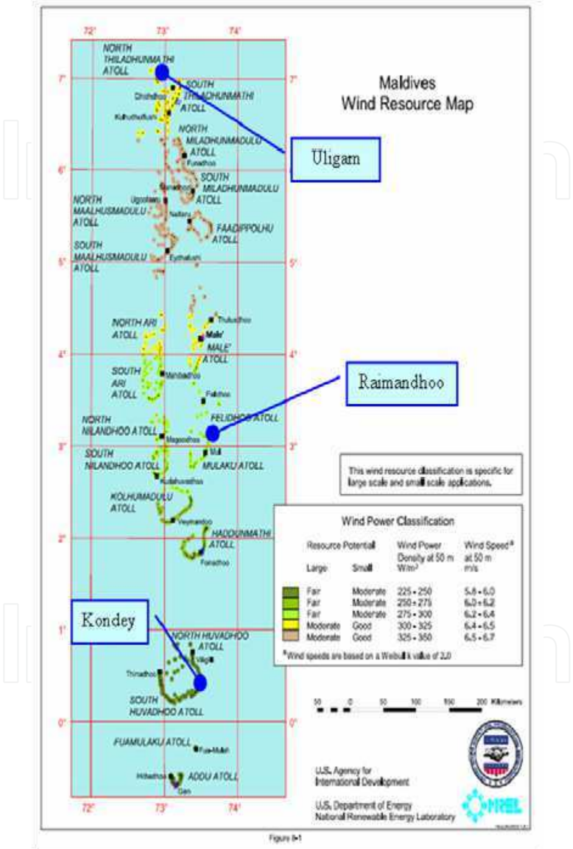
Fig. 6. Wind power resource and the selected islands
