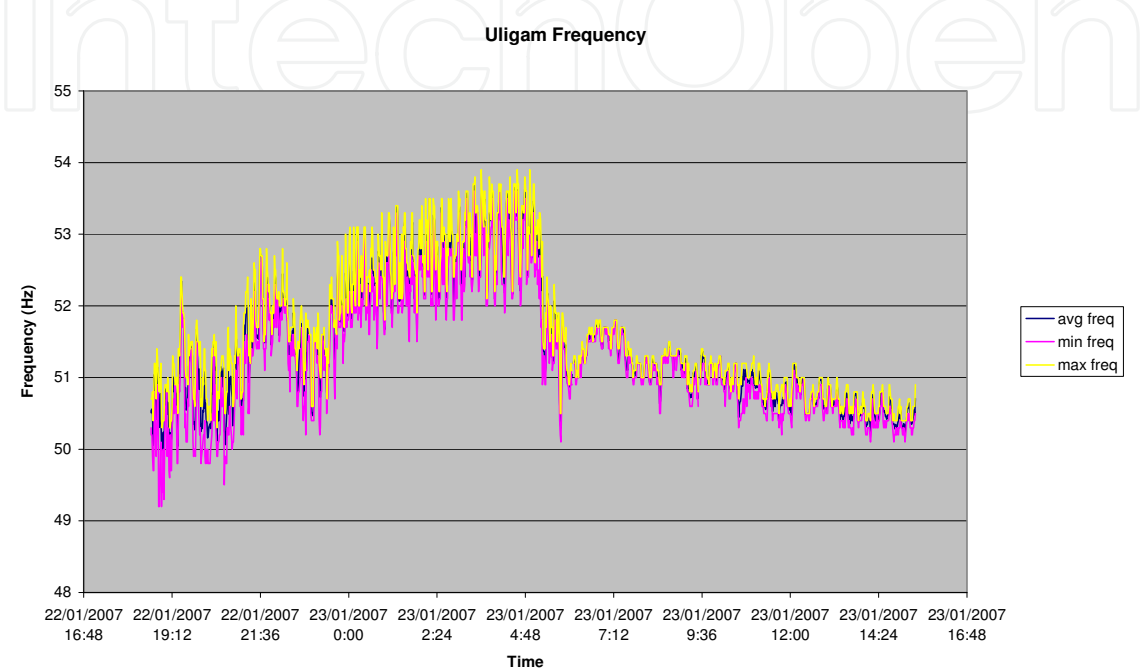
Fig. 9.b - Typical frequency data
