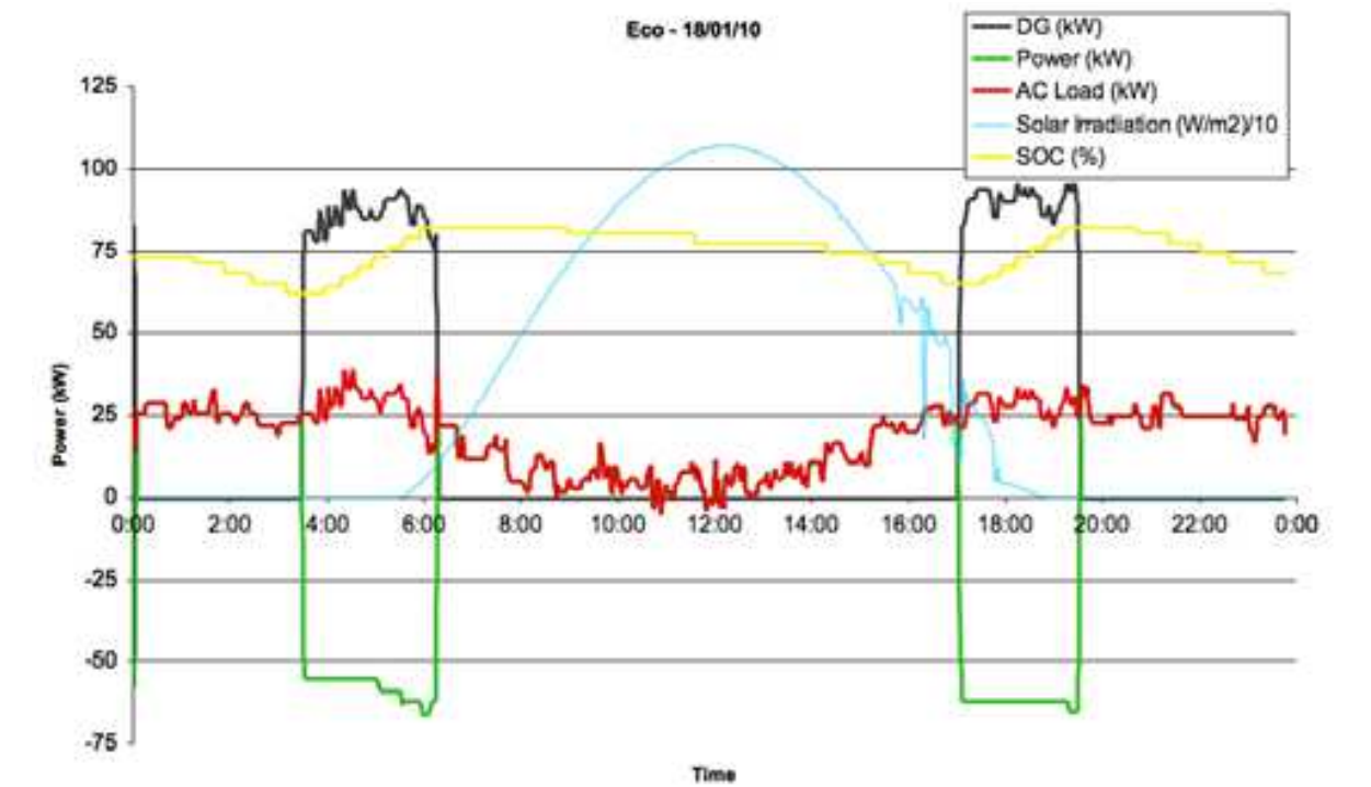
Fig. 21. System operation on a clear sunny day
