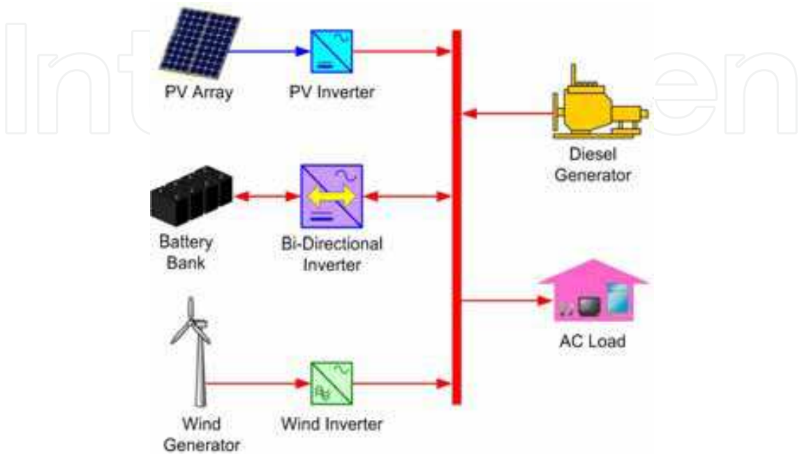
Fig. 4. Hybrid system schematic diagram showing renewable energy sources coupled to the ac side
