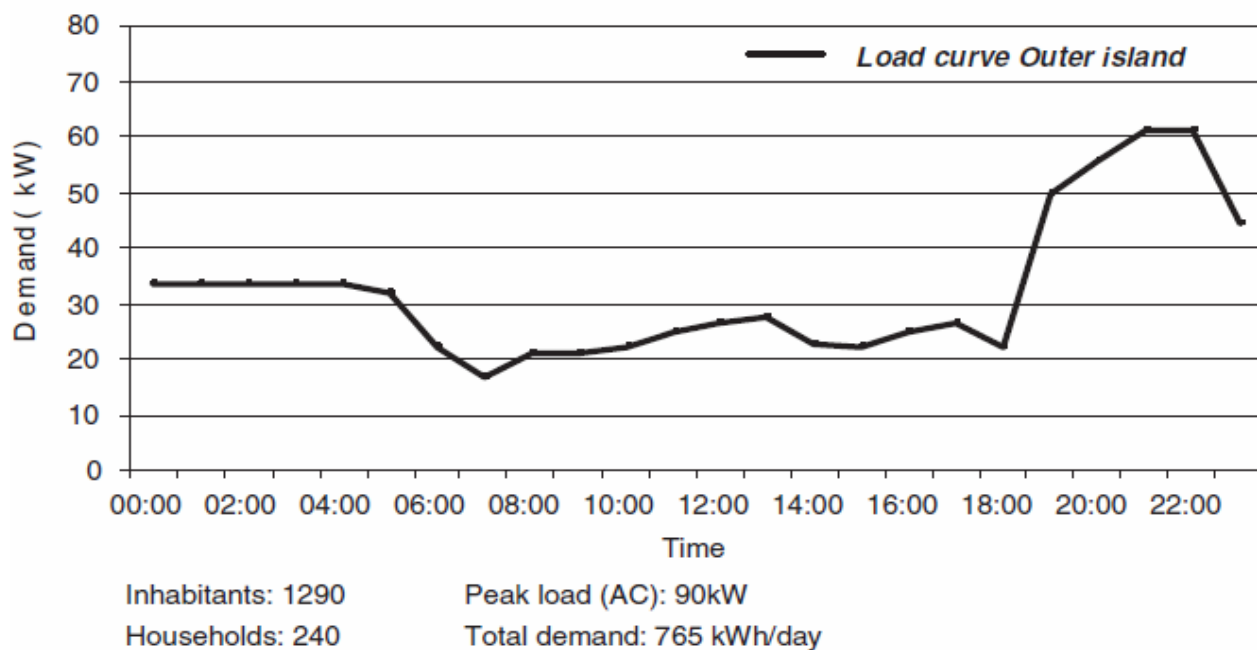
Fig. 10. Typical daily load profile
