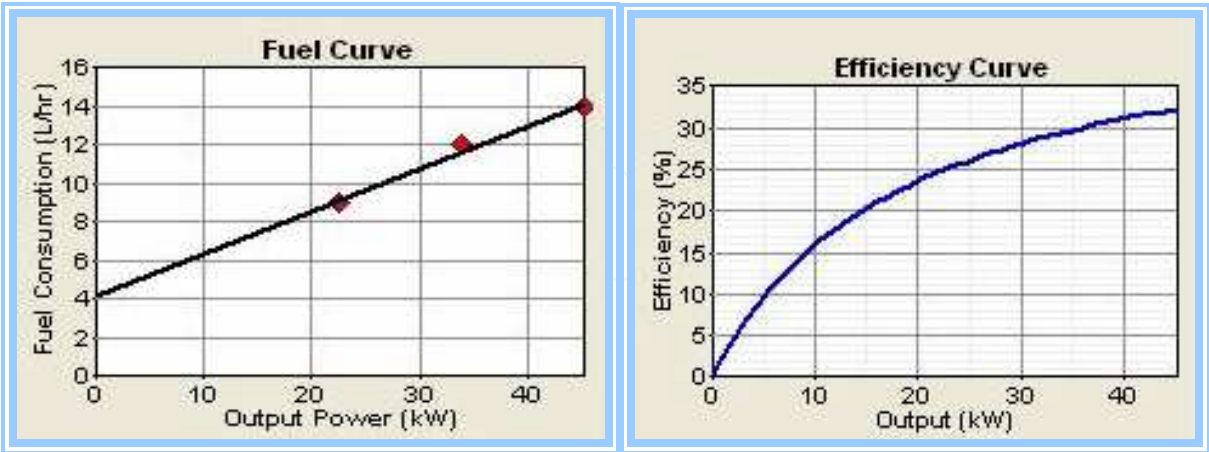
Fig. 2. Typical fuel consumption characteristics of diesel generator
