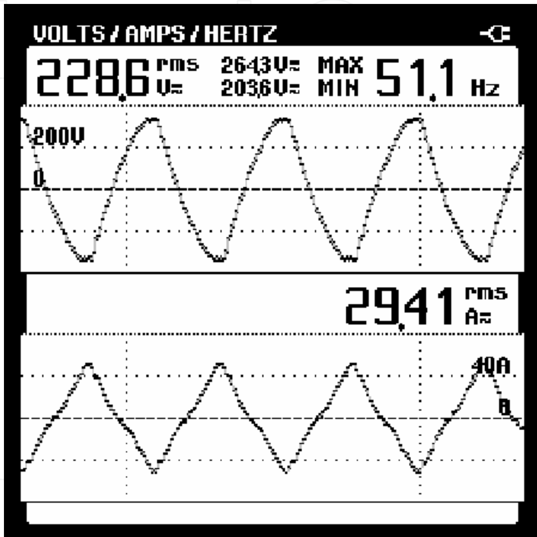
Fig. 9.a - Typical voltage and current waveforms
