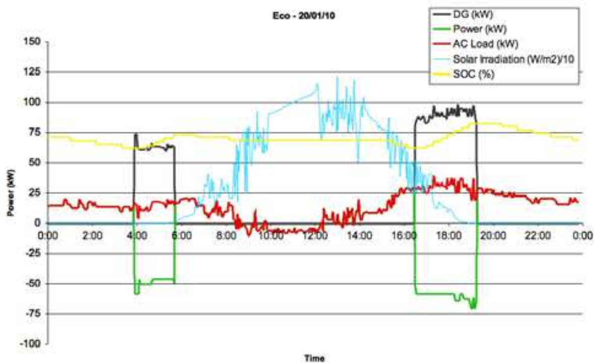
Fig. 22. System operation on a cloudy day
