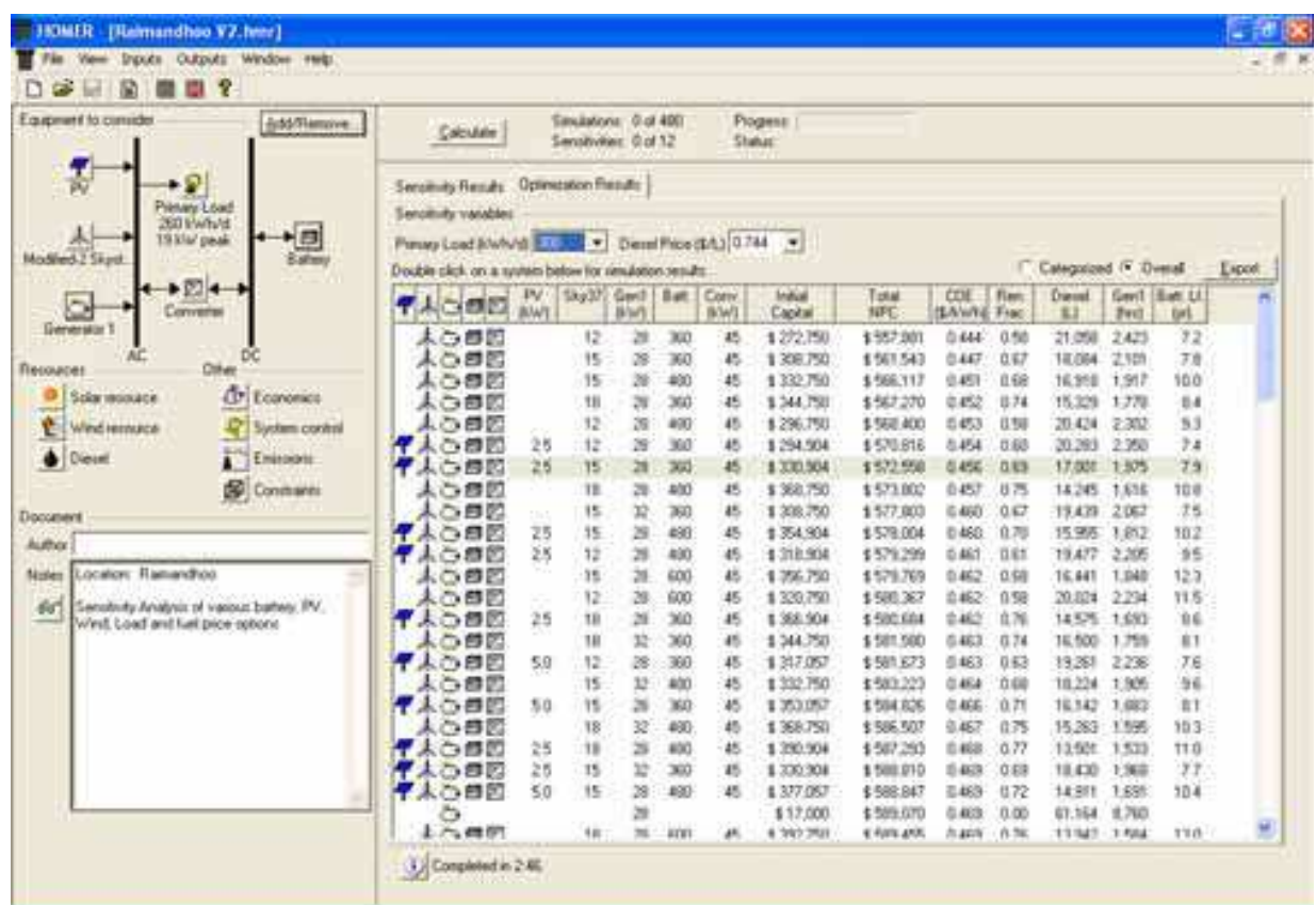
Fig. 12. Homer program output
