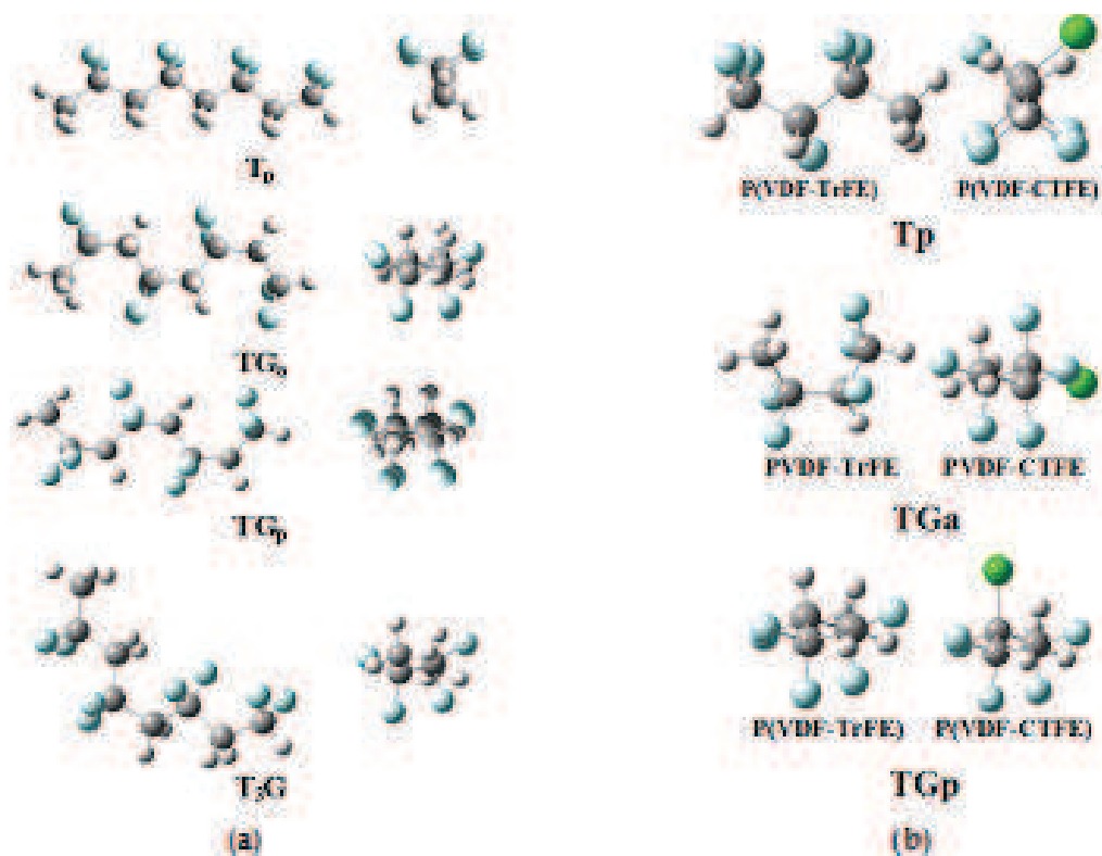
Fig. 1. Structural representation for the different PVDF conformers, namely, \text{T}_p , \text{TG}_a , \text{TG}_p and \text{T}_3\text{G} . Fluorine atoms are in blue, carbon atoms are in grey and hydrogen atoms are in white. a) PVDF b) P(VDF-TrFE) and P(VDF-CTFE).
