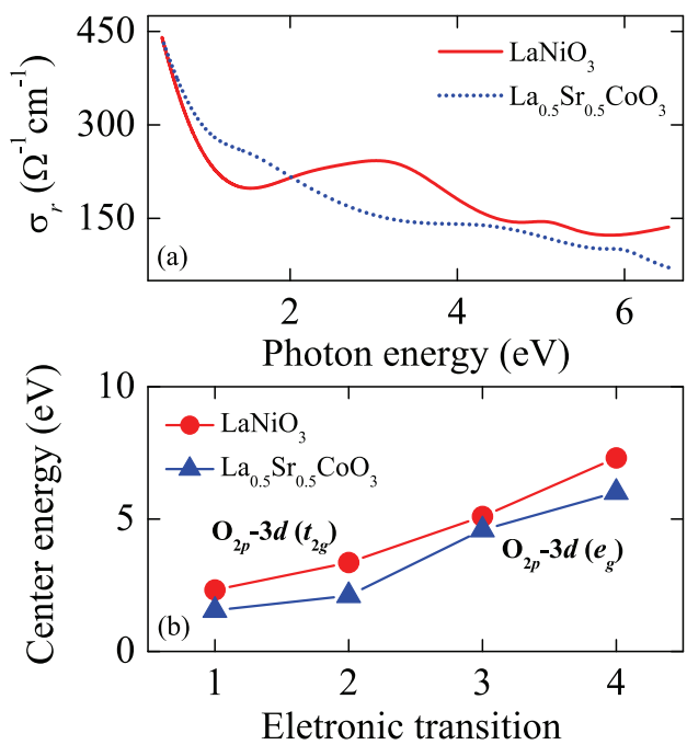
Fig. 9. The comparison of the optical conductivity between two films (a) and (b) the Lorentz oscillator E_j value corresponds to the electronic transitions from O 2p to Ni/Co 3d , respectively. (Figure reproduced with permission from (25). Copyright 2009, American Institute of Physics.)
