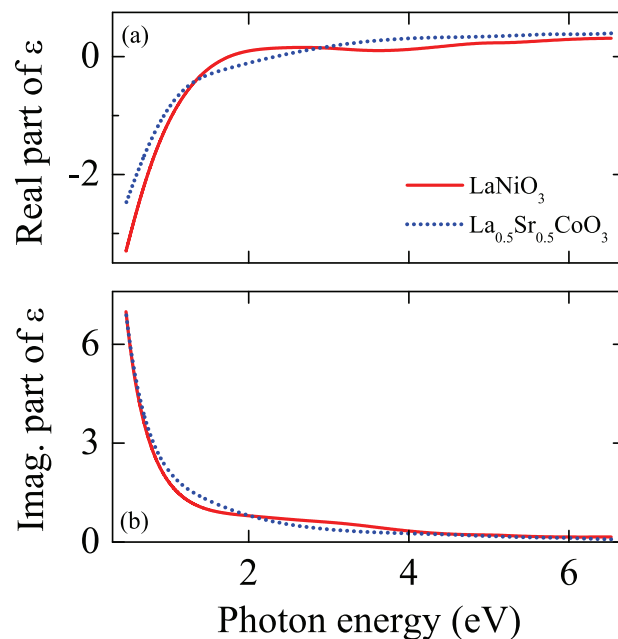
Fig. 8. The real part (a) and imaginary part (b) of dielectric function in \text{LaNiO}_3 and \text{La}_{0.5}\text{Sr}_{0.5}\text{CoO}_3 films from infrared to ultraviolet photon energy regions. (Figure reproduced with permission from (25). Copyright 2009, American Institute of Physics.)
