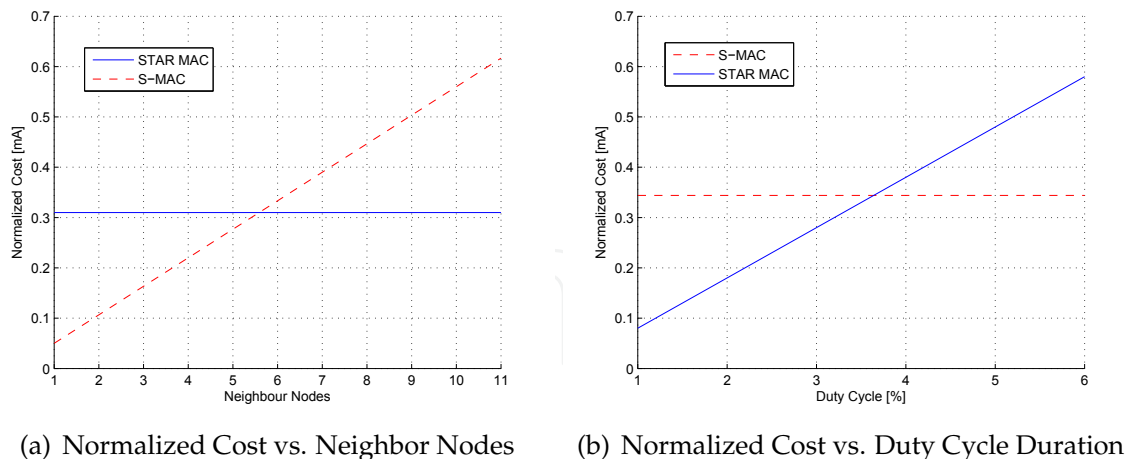
Fig. 5. STAR MAC Performance
