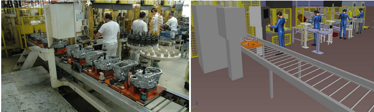
Fig. 10. DMUs of Assembly Workplace (Gregor,M.&Medvecky,S.,2010)
