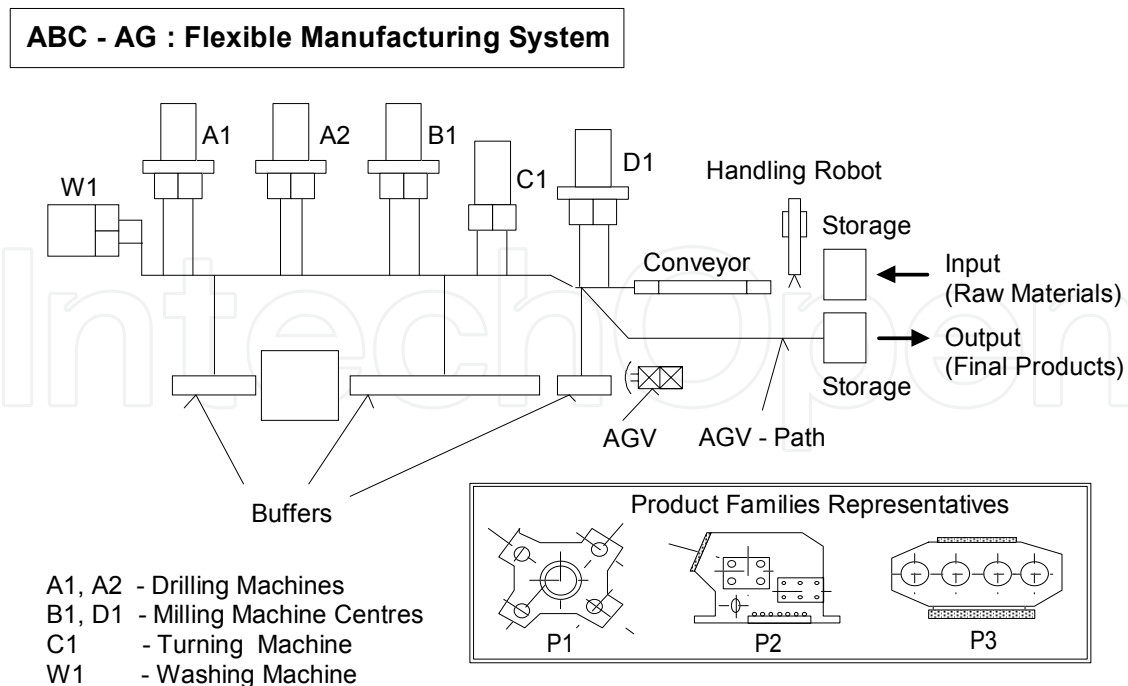
Fig. 16. Flexible Manufacturing System Layout (Gregor,M.&Kosturiak,J.,1997)
