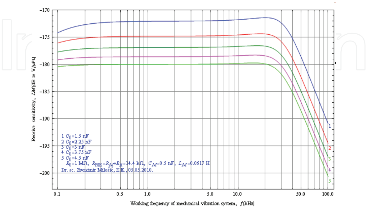
Fig. 4.3 Functional dependence of the level of the receive voltage sensitivity on the frequency at different parameters contained in mechanical, electric and acoustical part of transducer body calculated with given different numerical values of C_0 noticed inside figure By using Fig. 4.1 we can write equations for the next step, the step of matching electric impedance of hydroacoustical transducer as a hydrophone. Then we have
