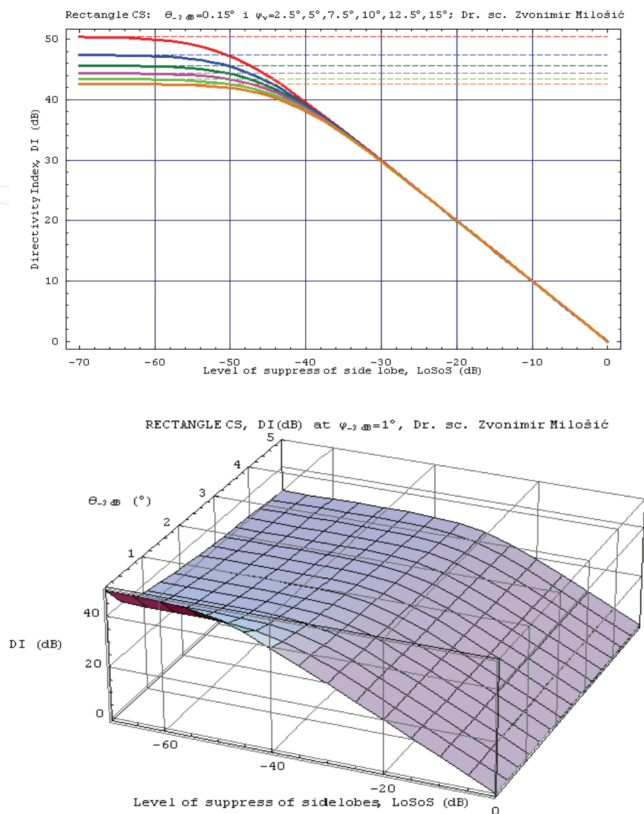
Fig. 6.1.2 Directivity index shown in two and three dimensions to (6.1.1) as correct function for theory and practice in dependence of LoSoS (dB) (Milošić 2004, 2005, 2007)
