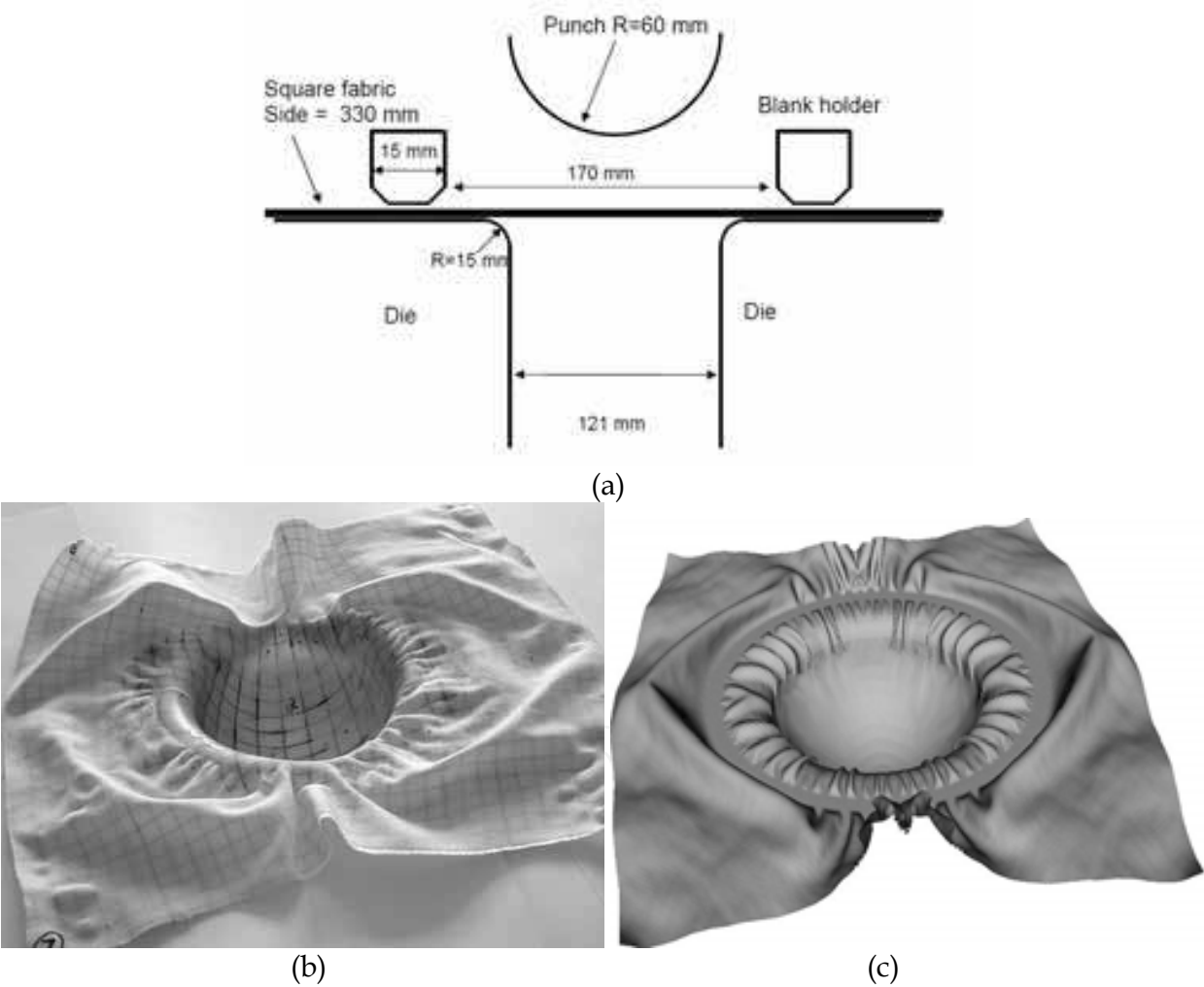
Fig. 21. Forming of an unbalanced textile reinforcement
